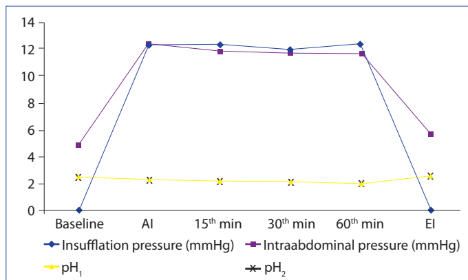
Figure 2. The relationships among IP, IAP, pH 1 , and pH 2 .
