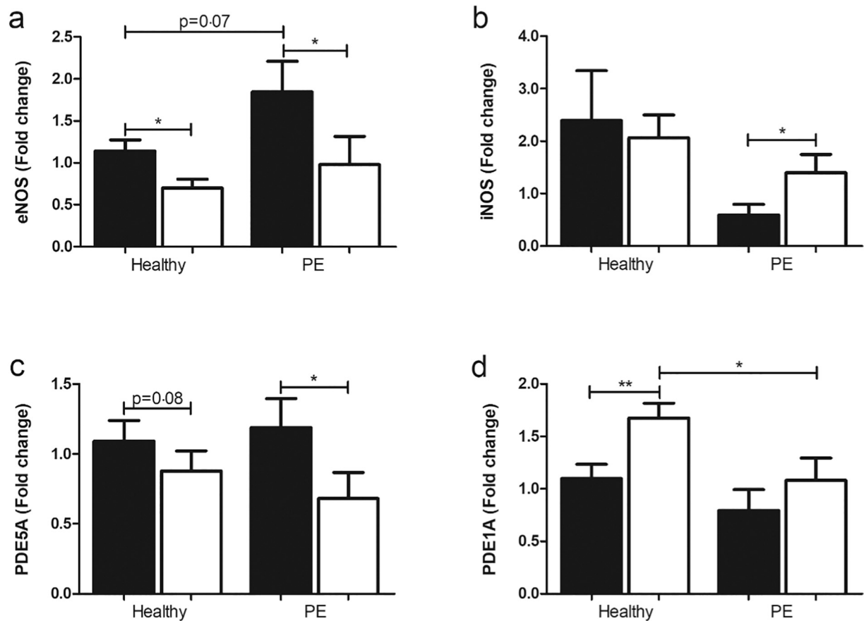
Fig. 3. mRNA expression. qPCR analysis of placental biopsies from the maternal (black bars) and foetal side (white bars) of 12 healthy and seven PE placentas. Data (mean \pm SEM) are expressed as fold change versus the maternal side biopsies of healthy controls. Panels a-d represent data for eNOS, iNOS, PDE5A and PDE1A. * p < 0.05 ; ** p < 0.01 (Mann-Whitney U test or Wilcoxon matched pairs test).
