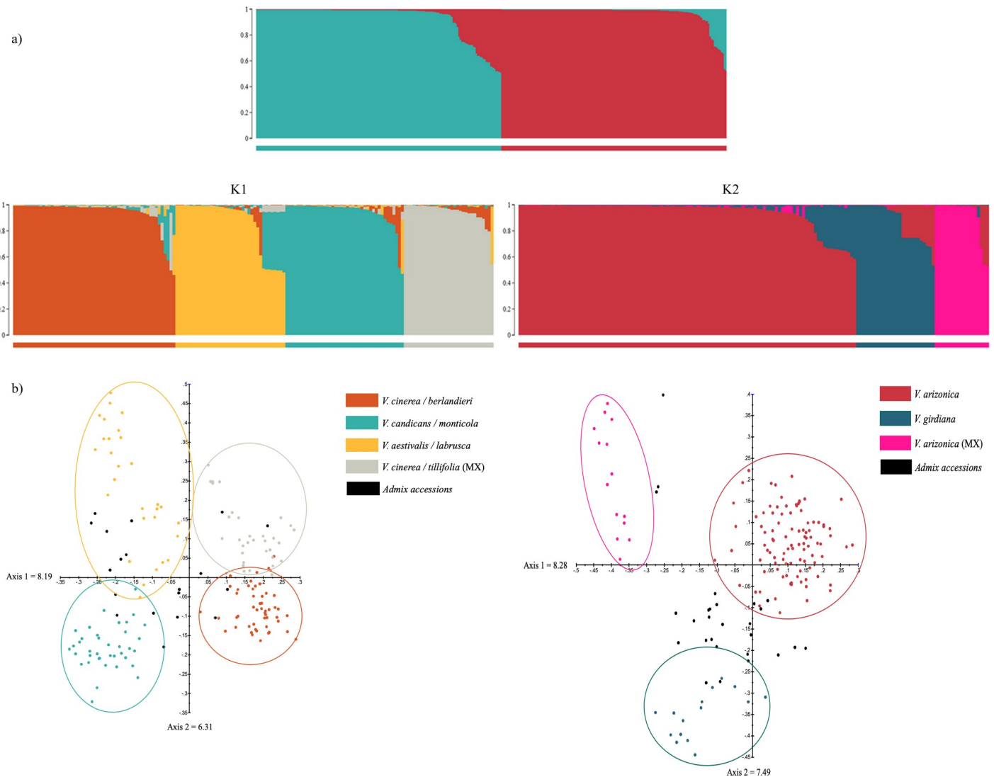
Fig 3. a) Bayesian STRUCTURE bar plot of membership for 326 accessions ( K = 2 ). Bright cyan represents group 1 ( K1 = southeastern US grape species) and moderate red represents group 2 ( K2 = southwestern US grape species). STRUCTURE analysis on each group resulted in four distinct sub-groups within K1 and three sub-groups within K2 . For details of membership coefficient values see S6 Table . b) Principal coordinate analysis for each group resulted in the comparable results to the Bayesian analysis. The color coding of the STRUCTURE assignment was used for the PCoA display.
