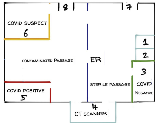
Fig. 4. A floor Plan of the Emergency Room of the Hospital divided into three zones.
