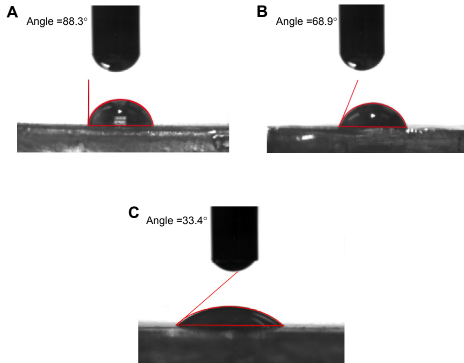
Figure 4 Representative contact angle images showing spreading of water droplet on control and coated mPE samples. Notes: (A) Pristine mPE, (B) 12 hours extract-coated mPE, (C) 24 hours extract-coated mPE. Abbreviation: mPE, metallocene polyethylene.
