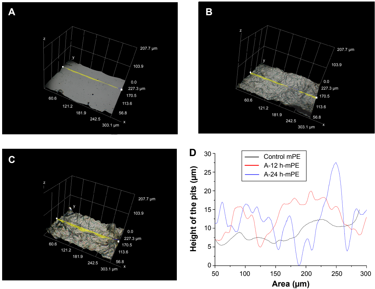
Figure 8 Hirox 3D images of control and extract-coated mPE samples taken at 1,000× with profiles.
