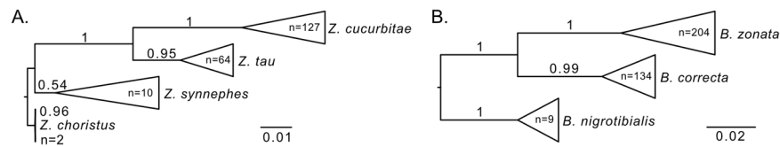
Figure 2. COI maximum likelihood trees based on unique haplotypes showing a monophyletic origin for (A) Zeugodacus cucurbitae and its closest congeners and (B) Bactrocera zonata and (B) correcta and their closest sister species. Scale bar indicates substitutions per site; the taxa are ‘collapsed’ into a triangle for each species, where the horizontal width indicates the maximum intraspecific variation. Bootstrap support values are indicated on the respective branches.
