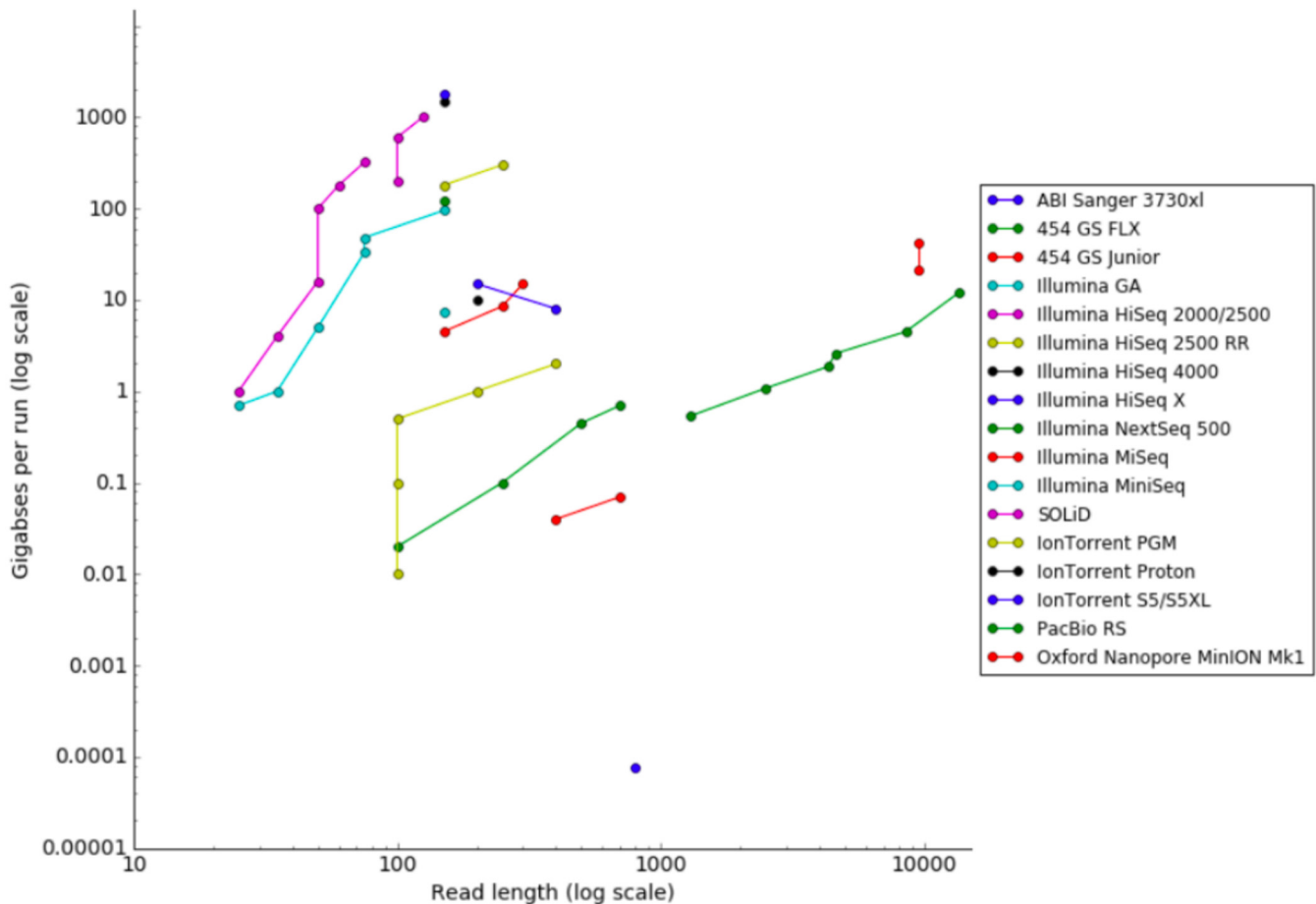
Figure 1. Timeline and comparison of different sequencing technologies. The data is based on the throughput metrics for the different platforms since their first instrument version came out. The figure visualises the results by plotting throughput in raw bases versus read length. Data released under CC BY 4.0 International license . doi 10.6084/m9.figshare.100940 .
