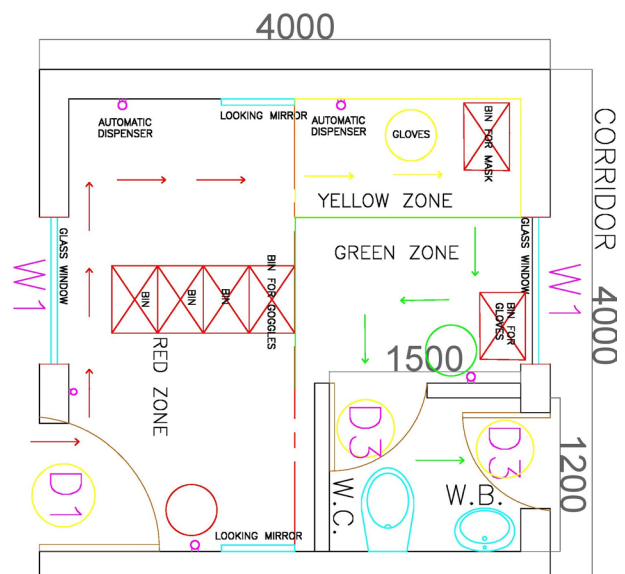
Figure 1 Size, layout and design of the doffing room.
