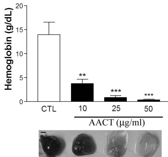
Figure 5. AACT inhibits VEGF-induced angiogenesis in mouse Matrigel-plug assay. Matrigel 500 µl containing 200 ng/ml VEGF with or without AACT (10, 25, 50 µg/ml) was subcutaneously injected into C57BL/5 C mice (5–9 mice/group). After 7 days, plugs were taken and photographed (Scar bar = 2 mm). Hemoglobin was measured as an indication of blood vessel formation, using the Drabkin method. Data are presented as mean ± S.E.M of at least 3 mice per group. ** P < 0.01 , *** P < 0.001 compared with control.
