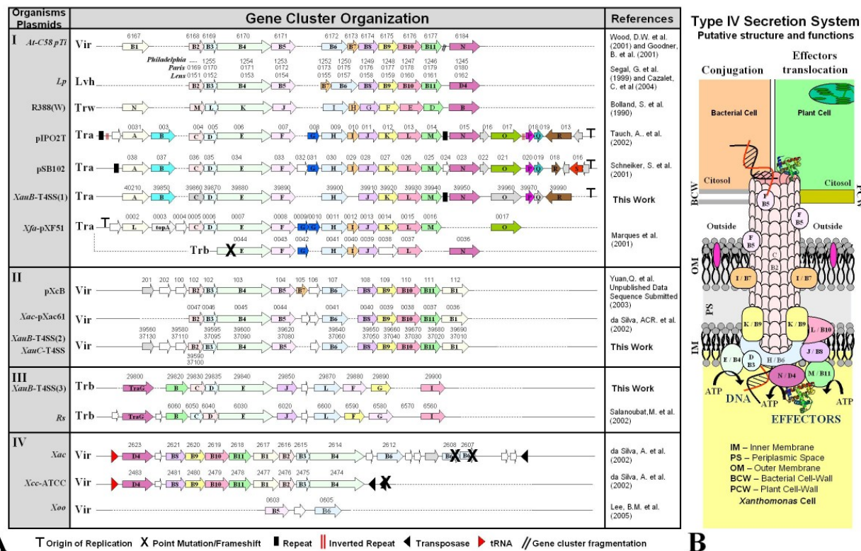
Figure 7 Schematic representation of Type IV Secretion System Genes in diverse bacteria, grouped by their genomic architecture. The colors used for gene arrows correspond to the colors used for their respective protein products in the secretion system representation on the right. At : Agrobacterium tumefaciens C58; Lp : Legionella pneumophila ; Xfa : Xylella fastidiosa 9a5c; Rs : Ralstonia solanacearum ; Xcc : Xanthomonas campestris pv. campestris ATCC33913; Xoo : Xanthomonas oryzae pv. oryzae . References not cited in the text are: Goodner et al. (2001) [113]; Segal et al. (1999) [114]; Cazalet et al. (2004) [115]; Bolland et al. (1990) [116]; Marques et al. (2001) [117]; Lee et al. (2005) [118].
