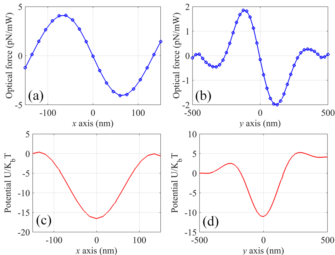
Figure 9. Optical force exerted on 100 nm (radius) resonant gold nanoparticle along (a) x- and (b) y-axis of the plasmonic tweezers working at 532 nm. Distribution of the corresponding potential depth along (c) x- and (d) y-axis for total input power of 200 mW.
