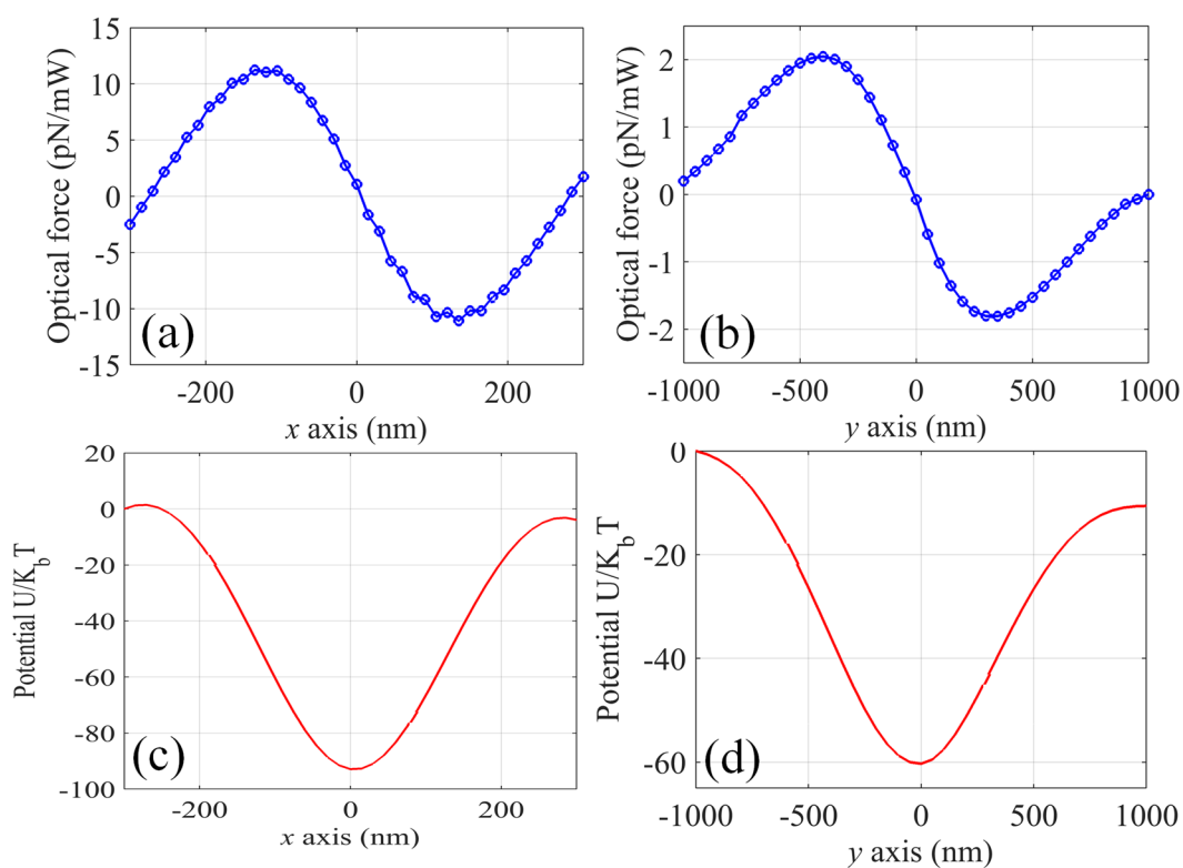
Figure 8. Optical force exerted on 100 nm (radius) gold nanoparticle along (a) x- and (b) y-axis of the plasmonic tweezers working at 1064 nm. Distribution of the corresponding potential depth along (c) x- and (d) y-axis for total input power of 200 mW.
