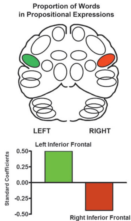
FIG. 3. The significant multiple linear progression predictors of the percentage of words in propositional expressions during spontaneous monologues. The standardized beta regression weights for left inferior frontal blood flow were positive, ( +0.51 ) whereas the regression weights for the right inferior frontal blood flow ( -0.44 ) were negative. This pattern represents the strong cerebral functional asymmetry for speech and language that is found after unilateral brain injury in right-handed individuals.
