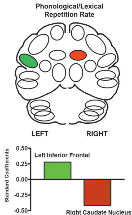
FIG. 1. The significant multiple linear regression predictors of speech rate during the repetition of phonological and lexical items. The standardized beta regression weight for left inferior frontal blood flow ( +0.28 ) increases while the regression weights for the right caudate nucleus decrease ( -0.41 ) as the rate of syllable production increases. This predictive pattern has been previously reported for normal and ataxic speakers.
