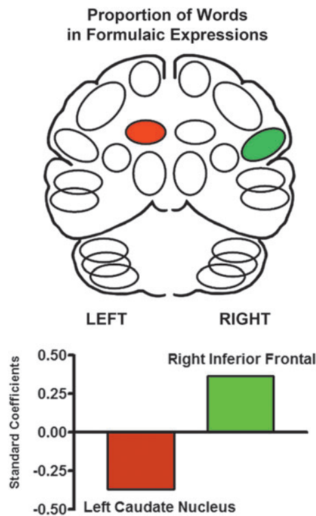
FIG. 2. The significant multiple linear progression predictors of formulaic expression use during spontaneous monologues. The standardized beta regression weight for left caudate blood flow was negative ( -0.37 ), whereas the regression weights for the right inferior frontal region ( +0.37 ) were positive. This pattern is complementary to the pattern found for syllable rate during the repetition of phonological and lexical items.
