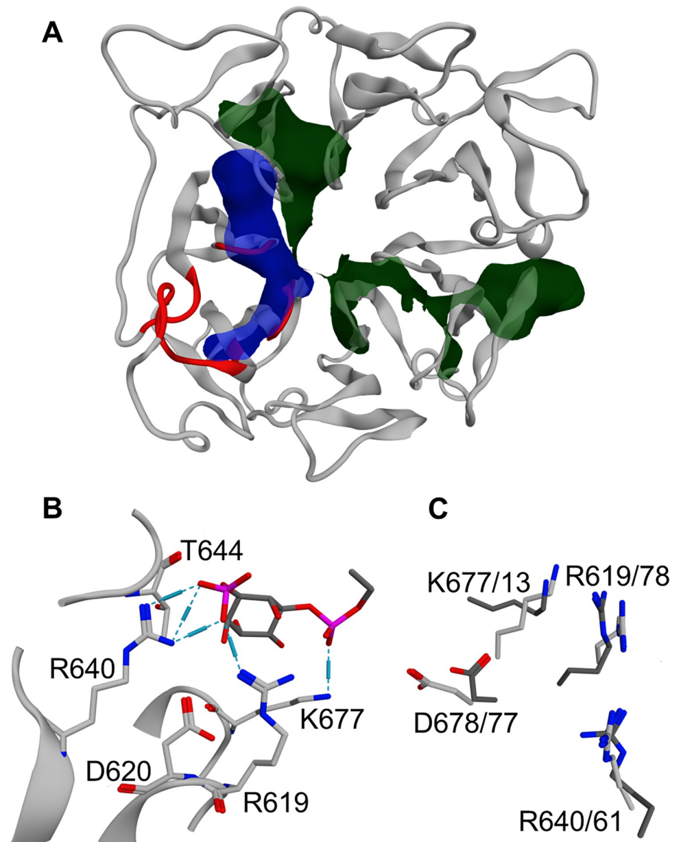
Fig 2. Identification of a putative PIP-binding site in Alsin RLD. (A) Visual rendering of the investigated binding pocket. The positive and hydrophobic surface patches are shown in blue and green, respectively, while residues forming the binding site are colored in red. (B) Binding pose of PI(3)P at the end of the dynamics, where interactions between two atoms are represented by dashed lines. The strength of an interaction is visually represented by the length of the cylinder. (C) Superimposition of RLD query residues (light grey) and the corresponding amino acids of the best hit found through ASSAM (dark grey). In the figure, residue numbers are reported according to the scheme N_{query}/N_{hit} .
