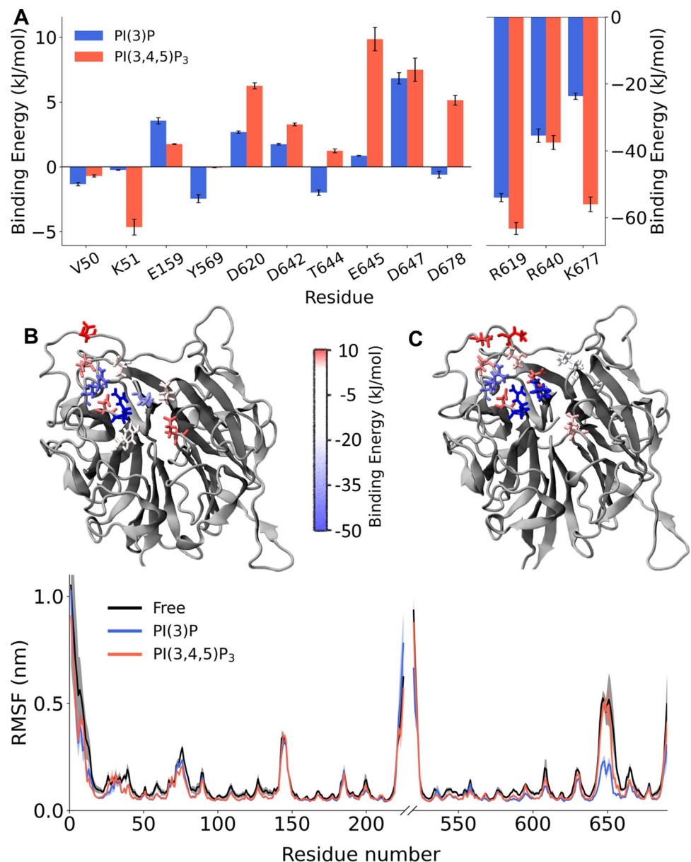
Fig 3. Comparison of RLD-PIPs interaction. (A) Decomposition of PI(3)P and PI(3,4,5)P 3 binding free energy, where error bars represent standard deviations. (B) Visual rendering of PI(3)P binding energy decomposition. (C) Visual rendering of PI(3,4,5)P 3 binding energy decomposition. (D) Comparison of RMSF values in absence and presence of PIPs. The shaded areas represent the standard deviation of the RMSF between the simulations. Loop L1, L2, and L3 are highlighted within the RMSF profile.
