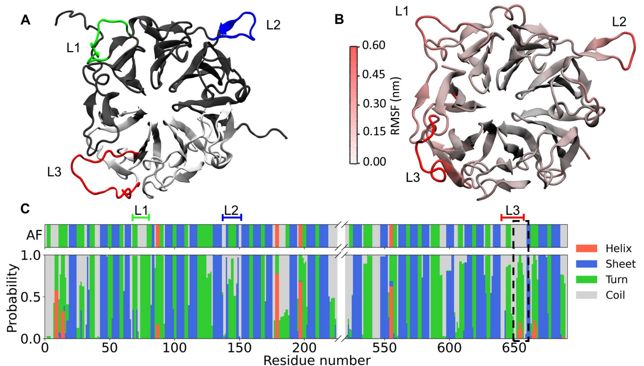
Fig 1. Alsin RLD structural refinement. (A) RLD^{AF} model is characterized by three loops protruding from the propeller, i.e. L1 (green), L2 (blue), and L3 (red). Chain A and B are colored in grey and white, respectively. (B) Refined Alsin RLD model. Residues are colored according to their RMSF to highlight in red the most flexible regions. For visualization purposes, the highly flexible N-terminal, aa. 220–225, and aa. 520–525 are not shown. (C) Secondary structure probability for each residue compared to the initial structure of RLD^{AF} . The region with increased turn probability after the dynamics is highlighted.
