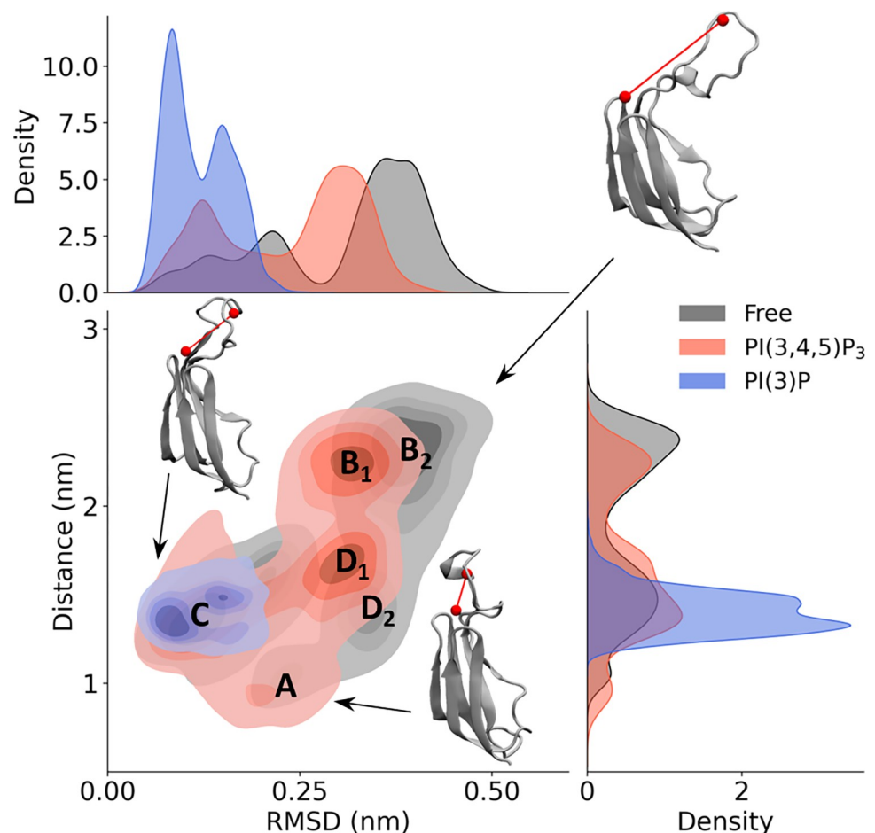
Fig 4. Analysis of L3 conformational dynamics. L3 dynamics has been described as RMSD from its position in the refined RLD model and distance from the investigated binding site. The probability distribution in the case of RLD alone, PI(3)P-bound RLD, and PI(3,4,5)P 3 -bound RLD is shown in black, blue, and red, respectively. Representative configurations of L3 are shown highlighting its distance from the binding pocket in red.
