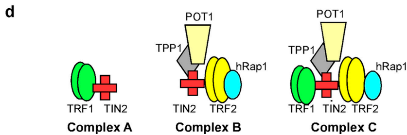
Figure 2. TIN2-mediated complexes. (a) Endogenous TIN2 complexes in HeLa nuclear lysate. Telomeric proteins in HeLa nuclear extracts (2.5 ml) were fractionated on a Sepharacryl S-300 HR column and immunoblotted for the indicated proteins. 20 \mu l aliquots of the indicated fractions were loaded. Eluting fractions were collected from the column after the void volume (No. 13). Molecular sizes indicated were derived from a standard curve based on the elution standards as described in Materials and methods. (b) Western blotting signals in Fig. 2 a were quantified with the Multi-Gauge program. Relative
