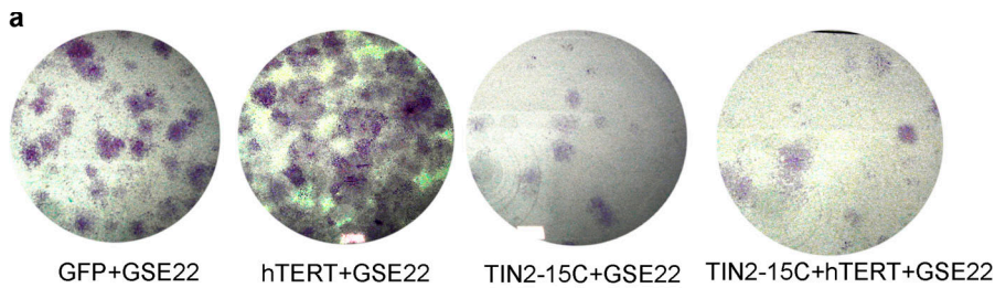
Figure 6. Effects of telomerase and a proposed model. (a) Telomerase does not rescue cell death by TIN2-15C. 5 \times 10^4 senescent cells were infected with lentiviruses expressing GFP (control), the telomerase catalytic subunit hTERT, TIN2-15C, or both TIN2-15C and hTERT. The cells were then infected with lenti-GSE-22. After 2 d, the cells were subcultured and plated for colony formation. Colonies were fixed and stained 61 d later. (b) Colonies were counted 5, 11, and 61 d after plating. Colonies were scored in two or three independent experiments for each transfection. Error bars represent the standard deviation. (c) Proposed model for TIN2 complexes at telomeres. Complex A and B cooperate, albeit at different positions on telomeres, to form t-loops or other terminal structures. Complex B may localize preferentially or uniquely near t-loop junctions, whereas A complexes may modulate the tertiary structure of telomeres and promote B complex stability. TIN2-13 disrupts complex A, thereby reducing the tertiary telomeric structure and destabilizing B complexes, resulting in partial or mild disruption of t-loops and telomere uncapping. TIN2-15C directly disrupts B complexes, resulting in severe disruption of t-loops and telomere uncapping. Cells expressing wild-type p53 and TIN2-13 or TIN2-15 undergo growth arrest, whereas cells lacking functional p53 undergo cell death. In both cases, the consequences of TIN2-15C expression are more severe than that of expressing TIN2-13.
