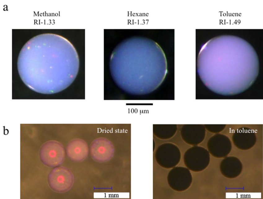
Figure 9 | Photographs of the glossy secondary particles under solvents. (a) Secondary particles composed of 360-nm silica particles in different solvents. (b) Secondary particles composed of 360-nm silica particles with CB in the dried state and in toluene.
