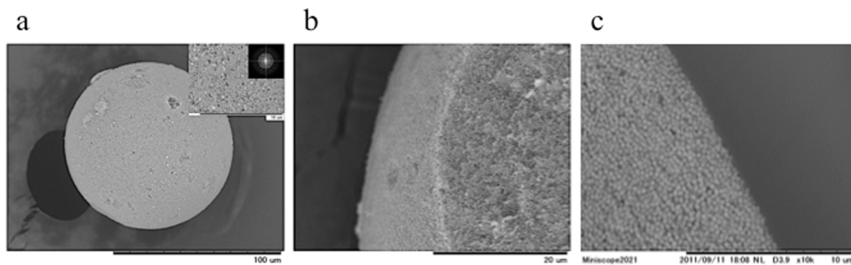
Figure 6 | Microstructures of the matte secondary particles. (a) An SEM image of a matte secondary particle composed of 360-nm silica particles. The inset presents a magnification of the SEM image and the FT image. (b) A cross-sectional SEM image of a matte secondary particle prepared by grinding the matte secondary particle in liquid nitrogen. (c) A cross-sectional SEM image of the matte secondary particle prepared by microtoming the embedded sample.
