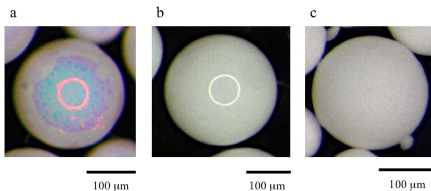
Figure 1 | Photographs of the secondary particles. (a) A secondary particle composed of silica particles 360 nm in diameter viewed under a microscope. (b) A secondary particle composed of silica particles 280 nm in diameter viewed under a microscope. (c) A secondary particle composed of silica particles 360 nm in diameter prepared with the addition of NaCl.
