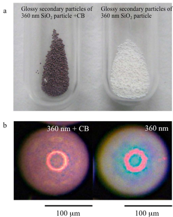
Figure 2 | Photographs of the glossy secondary particles with and without CB. (a) Secondary particles composed of silica particles 360 nm in diameter and CB (left). Secondary particles composed of silica particles 360 nm in diameter (right). (b) A secondary particle composed of silica particles 360 nm in diameter and CB (left). A secondary particle composed of silica particles 360 nm in diameter (right).
