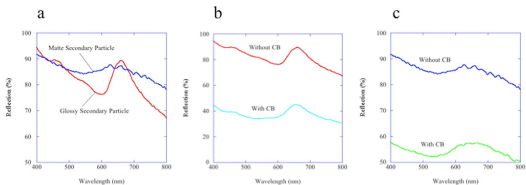
Figure 7 | Reflection spectra of the secondary particles. (a) Reflection spectra of the glossy and matte secondary particles composed of 360-nm silica particles. (b) Reflection spectra of the glossy secondary particles composed of 360-nm silica particles with and without CB. (c) Reflection spectra of the matte secondary particles composed of 360-nm silica particles with and without CB.
