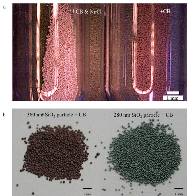
Figure 4 | Photographs of the secondary particles with CB prepared with and without NaCl. (a) Secondary particles composed of silica particles 360 nm in diameter and CB, which were prepared with and without NaCl. (b) Secondary particles composed of silica particles 360 nm in diameter and CB (left). Secondary particles composed of silica particles 280 nm in diameter and CB (right).
