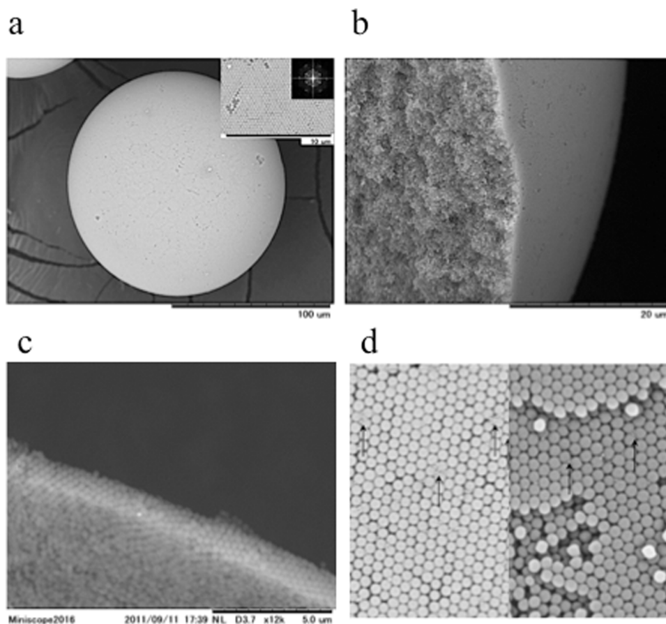
Figure 5 | Microstructures of the glossy secondary particles. (a) An SEM image of a glossy secondary particle composed of 360-nm silica particles. The inset presents a magnification of the SEM image and the FT image. (b) The cross-sectional SEM image of the glossy secondary particle prepared by grinding the glossy secondary particle in liquid nitrogen. (c) A cross-sectional SEM image of a glossy secondary particle prepared by microtoming the embedded sample. (d) SEM image of the surface of a glossy secondary particle. The CB is indicated by arrows.
