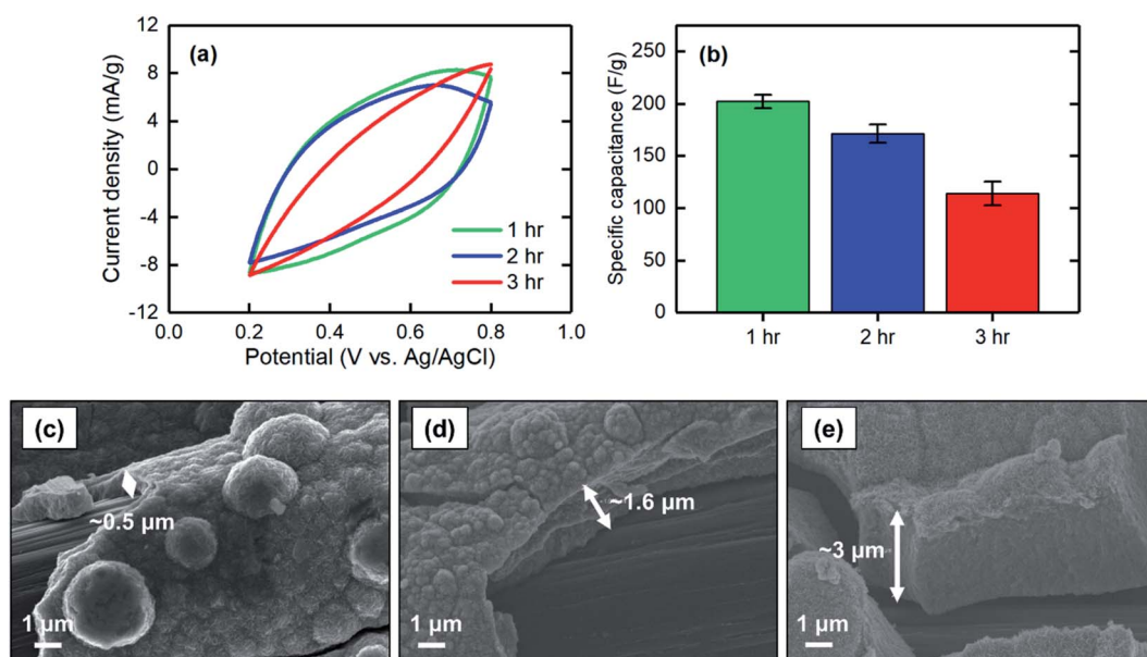
Fig. 6 (a) CV at a scan rate of 2 \text{ mV s}^{-1} , (b) corresponding specific capacitance, and SEM images of the \text{MnO}_2 electrodes electrodeposited at 1 \text{mA cm}^{-2} for (c) 1 hour, (d) 2 hours, and (e) 3 hours.
