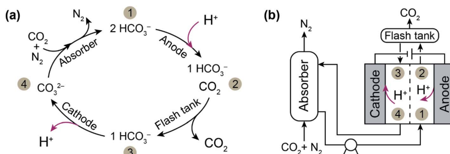
Fig. 1 (a) The chemical (black arrows) and electrochemical (red arrows) reactions of \text{CO}_2 capture with \text{K}_2\text{CO}_3 (denoted \text{CO}_3^{2-} ) as the absorbent and (b) a schematic diagram of the electrochemically driven proton concentration process. After the absorption stage, the stream is sent to the anode compartment of the electrochemical cell, where proton deintercalation from the electrode shifts the \text{CO}_2 (aq)/ \text{HCO}_3^- (aq)/ \text{CO}_3^{2-} (aq) equilibrium toward \text{CO}_2 formation ( i.e. , 1 \rightarrow 2), and this is followed by gas separation through a flash tank ( i.e. , 2 \rightarrow 3). Subsequently, the absorbent is regenerated in the cathode compartment, where proton intercalation occurs ( i.e. , 3 \rightarrow 4).
