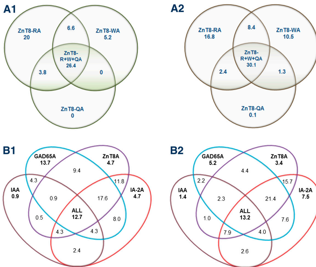
FIG. 2. Venn diagrams of islet autoantibodies. A: Frequencies and codetection (percent positive) of ZnT8A in A1: non-Swedes ( n = 212 ) and A2: Swedes ( n = 2,160 ). B: ZnT8A ( \geq 1 ZnT8 autoantibodies) were detected in 4.7% of non-Swedes ( B1 ) and 3.4% of Swedes ( B2 ) who were negative for conventional autoantibodies. Unlike Swedes, non-Swedes develop ZnT8A more frequently with GAD65A rather than IA-2A. (A high-quality color representation of this figure is available in the online issue.)
