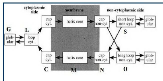
Figure 1: Architecture of TMHMM consists of 7 boxes and each box indicates the particular region. Same text box treats as same region. Here we have denoted each box by symbols to its corresponding region. Each box may be one or more states in HMM with same parameters.
