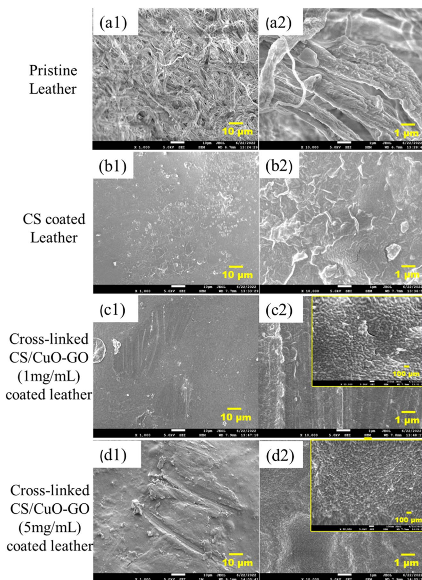
Fig. 4 FE-SEM images of pristine leather (a1 and a2), chitosan-coated leather (b1 and b2), CS/CuO-GO ( 1\text{ mg mL}^{-1} ) coated leather (c1 and c2), and CS/CuO-GO ( 5\text{ mg mL}^{-1} ) coated leather (d1 and d2) samples at different magnifications ( 1000\times and 10\,000\times ). Insets show magnified images ( 50\,000\times ), indicating the presence of CuO-GO nanostructure on the leather surface.
