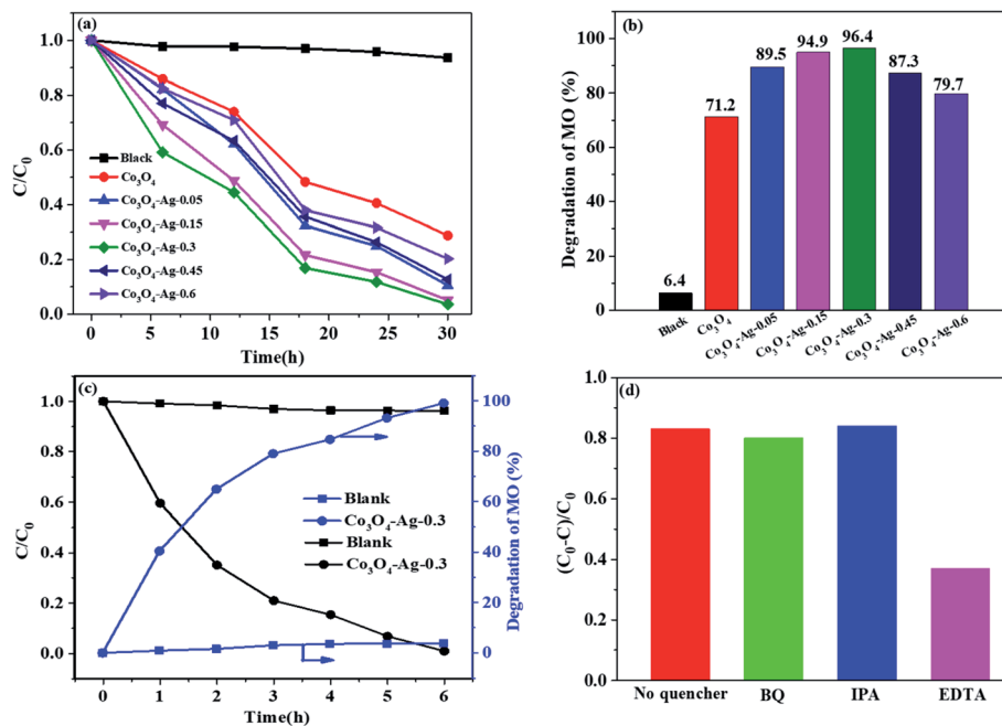
Fig. 8 Degradation rate (a) and degradation efficiency of MO in 30 h (b) over the series of catalysts under UV light. Photocatalytic degradation of MO with or without \text{Co}_3\text{O}_4\text{-Ag-0.3} under visible light (c). Trapping experiments of the active species during the photocatalytic degradation of MO with \text{Co}_3\text{O}_4\text{-Ag-0.3} under UV radiation (d).
