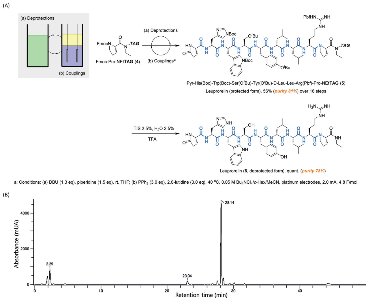
Scheme 2 (A) Biphasic electrochemical synthesis of leuprorelin, and (B) HPLC analysis of leuprorelin (protected form, R. T. = 28.14) (5).
