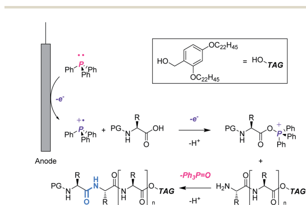
Fig. 1 Electrochemical peptide synthesis utilizing soluble tag-assisted method.
