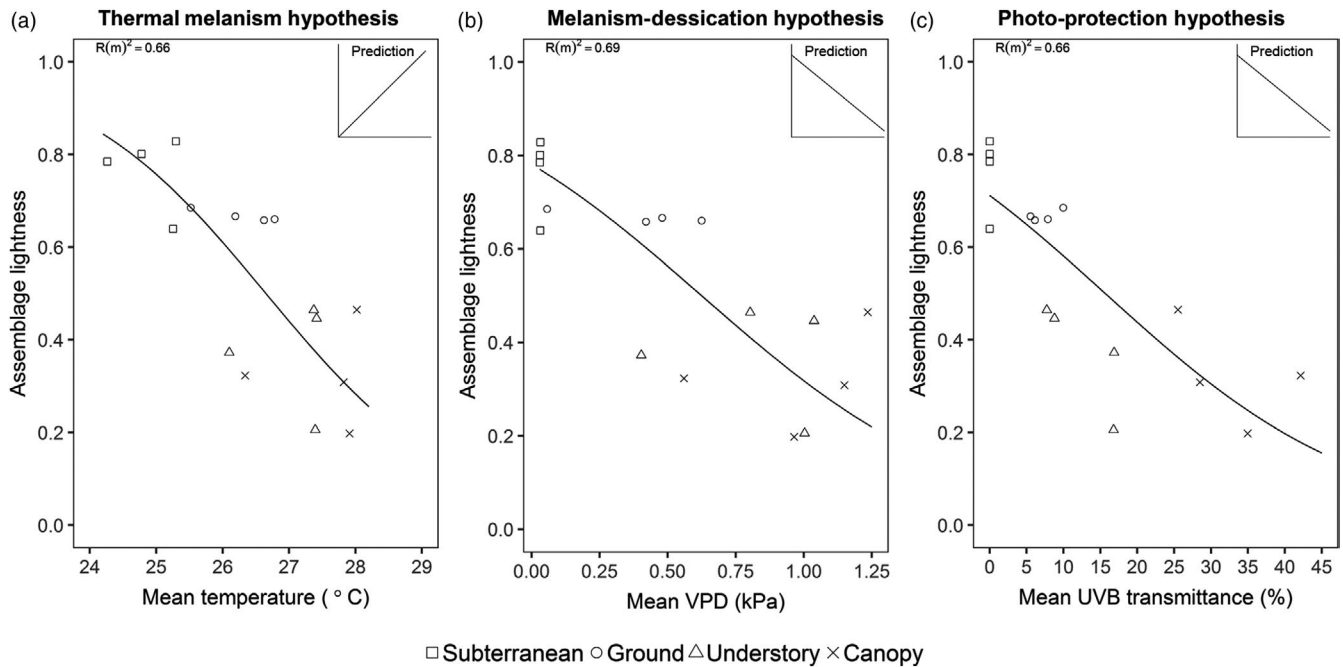
FIGURE 5 Relationship between assemblage-weighted lightness and (a) mean temperature, (b) mean vapour pressure deficit (VPD) or (c) mean UV-B transmittance. Lines display model predictions and R m 2 (fixed effects) are shown. For subterranean stratum, VPD was calculated by assigning a humidity value of 99% to each subterranean assemblage while UV-B transmittance was assigned as 0% (n = 16 assemblages; 4 plots × 4 strata). Inset shows predicted relationship
