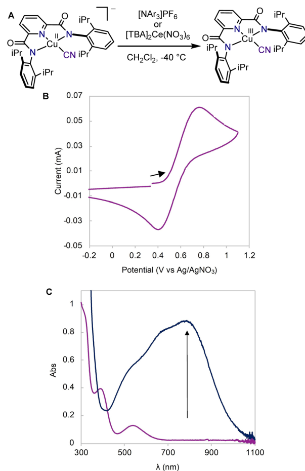
Fig. 1 (A) Synthesis of LCu III CN. (B) Cyclic voltammogram of [TBA]LCu II CN (3 mM in CH 2 Cl 2 with 0.1 M [TBA]ClO 4 at 23 °C). (C) UV-vis spectra showing the formation of LCu III CN (dark blue trace) by chemical oxidation of [TBA]LCu II CN (purple trace) in CH 2 Cl 2 at –40 °C.
