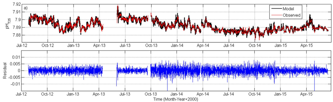
Figure 3. (a) \text{pH}_{T25} obtained with the SAMI device averaged to 84 h (red line) and modelled \text{pH}_{T25} (black line), (b) Residuals between observed values and modelled outputs.
