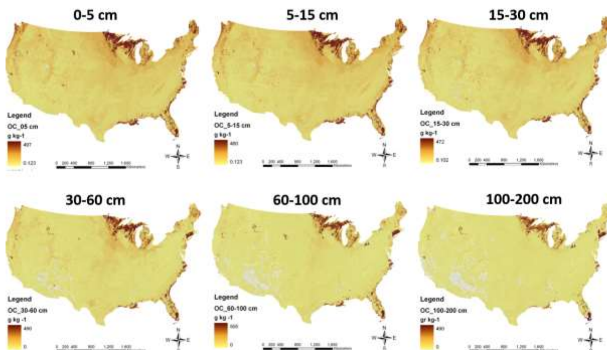
Figure 8. Maps of mean soil organic carbon ( \text{g.kg}^{-1} ) at the 6 standard depths for continental USA.
