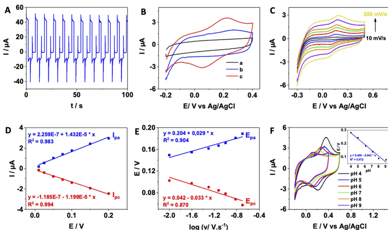
Fig. 1 (A) Electrochemical deposition and characteristics of the polydopamine film. I-t curve of first 100 s of the pulse deposition (30 pulse cycles) of 1 mg mL -1 of dopamine in 10 mM PBS (pH 7.0) at AuNPs/SPCE. (B) CV of SPCE (a), AuNPs/SPCE (b) and pDA/AuNPs/SPCE (c) in 0.01 M PBS (pH 7.0) at 100 mV s -1 . (C) CVs of pDA/AuNPs/SPCE in 0.01 M PBS (pH 7.0) at different scan rates (from inner to outer: 10–200 mV s -1 ); (D) plots of anodic and cathodic peak currents vs. scan rate of pDA/AuNPs/SPCE in 0.01 M PBS (pH 7.0). (E) Plots of peak potentials vs. logarithm of the scan rate for the pDA/AuNPs/SPCE in 0.01 M PBS (pH 7.0). (F) CVs of pDA/AuNPs/SPCE in 0.01 M PBS at different pH (inset: plot of the formal potential vs. pH value).
