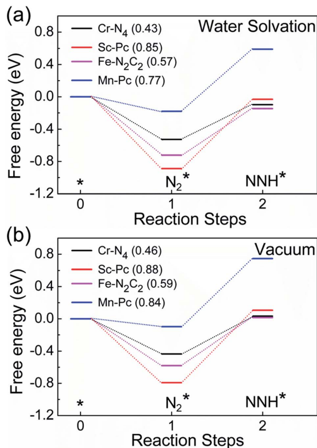
Fig. 6 Computed free energy profiles of \text{N}_2 and NNH adsorption on Cr- \text{N}_4 , Sc-Pc, Fe- \text{N}_2\text{C}_2 , and Mn-Pc in (a) the presence of an aqueous solvent and (b) vacuum. The corresponding values of overpotential are given in parentheses in the figure legends.
