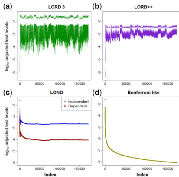
Fig. 1. Adjusted significance thresholds on the log 10 scale. Applied to genotype effect data from the IMPC dataset, at a FDR level of 5%. (a) LORD 3, (b) LORD++, (c) LOND and (d) Bonferroni-like
