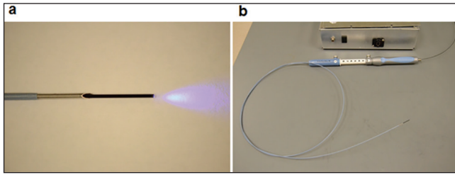
Figure 1. (a and b) Photographs of high-resolution microendoscope fiber-optic probe with 0.45-mm diameter passed through an EUS-guided FNA needle (Echotip ultra 19-gauge; Cook)
