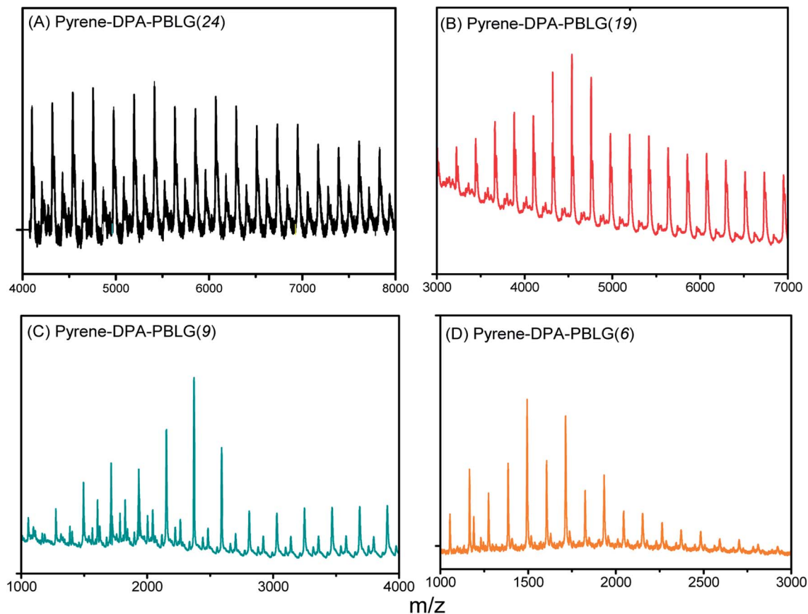
Fig. 4 MALDI-TOF mass spectra of (A) pyrene-DPA-PBLG(24), (B) pyrene-DPA-PBLG(19), (C) pyrene-DPA-PBLG(9), and (D) pyrene-DPA-PBLG(6).
