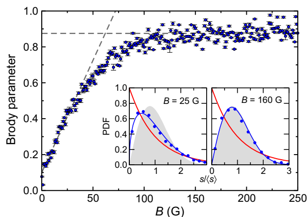
Fig. 6. Brody parameter \eta extracted from the NNSD as a function of B for weakly bound states with binding energy less than |\mathcal{E}|/\hbar = -0.5 GHz. The dashed gray lines extrapolate the linear small and large B -field behavior. Their crossing defines a transition strength. Insets show the NNS probability distributions (blue filled circles) for B = 25 and 160 G as a function of the normalized energy spacing s/\langle s \rangle , with mean spacing \langle s \rangle obtained for each B . Solid blue lines are Brody distributions fit to the data. Gray shaded areas and red curves indicate the Wigner-Dyson ( \eta = 1 ) and Poisson ( \eta = 0 ) distributions, respectively.
