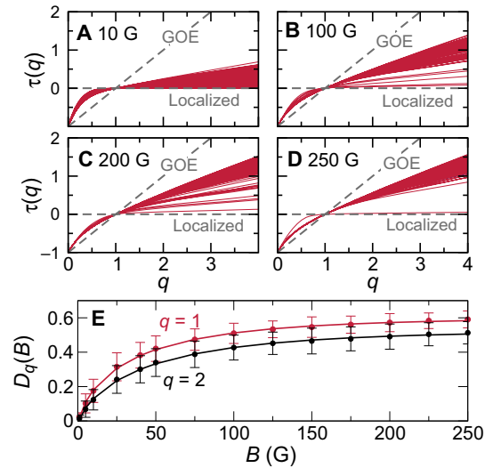
Fig. 4. Grand potential and fractal dimension of the weakly bound Dy_2 wave functions. (A to D) \tau(q) as a function of q for all weakly bound eigenstates (dark red curves) within an |\mathcal{E}/h| = 500 MHz energy range below the threshold at B = 10, 100, 200, and 250 G, respectively. The corresponding eigenenergies for these four B fields are shown in Fig. 3. The two dashed straight lines correspond to \tau(q) of the ergodic GOE and localized limits, respectively. (Although not shown, the curves remain concave for q < 0 .) (E) Fractal dimension D_q(B) , defined in the text, as functions of B for q = 1 and 2. The error bars indicate the spread of fractal dimension. Solid lines are for guiding the eye. For q = 1 and 2, the parameter d_0 = 0.57 and 0.49 , respectively.
