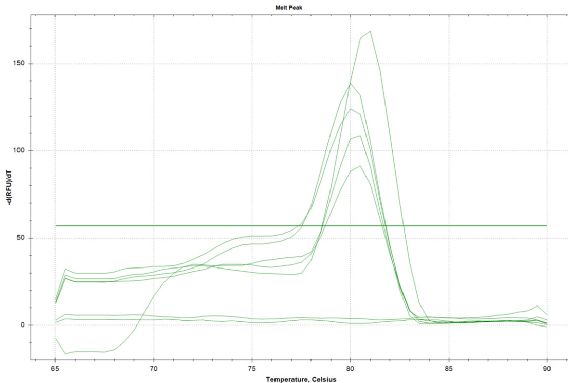
Figure 3. qPCR results. Melting peaks (plotted as the negative derivate of fluorescence F vs. T) analysis from a qPCR assay based on SYBR-green fluorescence for detection of PERVs. The dissociation temperature range extends from 65 to 90 °C. Melting peaks for the PERVs positive controls range 81.0 \pm 0.5 °C. Melting peaks for the paraffin embedded lymph node samples range 80.5 \pm 0.5 °C. No melting curve graphs are observed for negative control (human cell line) and NTC.
