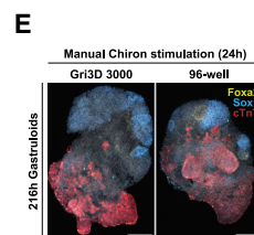
Figure 3E. Developmental potential of 3D gastruloids in response to time-varying Chir stimulation (original)
