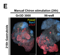
Figure 3E. Developmental potential of 3D gastruloids in response to time-varying Chir stimulation (corrected)
