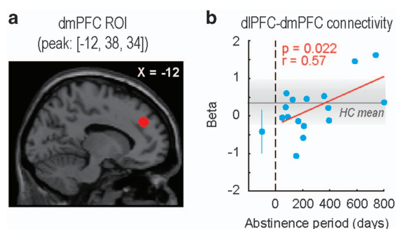
Figure 4. Functional connectivity analysis with left dlPFC seed. (a) Red-filled circle on a sagittal slice indicates dmPFC ROI (peak coordinates: [-12, 38, 34]). (b) Relationship between abstinence period (abscissa) and dmPFC ROI response (ordinate). Beta represents the regression coefficient of GLM regarding ‘strategy optimization’ contrast ([-1 0 1 1 -1]). Schema of the figure is the same as Figures 2d–f. dlPFC, dorsolateral prefrontal cortex; dmPFC, dorsomedial prefrontal cortex; GLM, general linear model.
