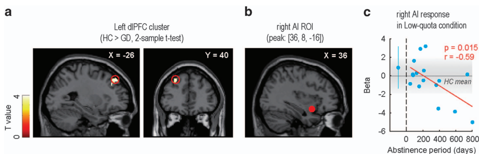
Figure 3. Activation analysis. (a) Result of two-sample t -test using quota severity contrast ([0 -2 -1 1 2]). Red open circles indicate left dlPFC cluster on a sagittal slice (left) and on a coronal slice (right). The peak coordinates were at [-26, 40, 44]. The threshold was set at P < 0.05 with cluster-size correction. (b) Red-filled circle on a sagittal slice indicates right AI ROI (peak coordinates: [36, 8, -16]). (c) Relationship between abstinence period (abscissa) and right AI ROI response in low-quota condition (ordinate). Beta represents the regression coefficient of GLM regarding single contrast of low-quota condition ([0, 0, 1, 0, 0]). Schema of the figure is the same as Figures 2d–f. AI, anterior insula; dlPFC, dorsolateral prefrontal cortex; GLM, general linear model.
