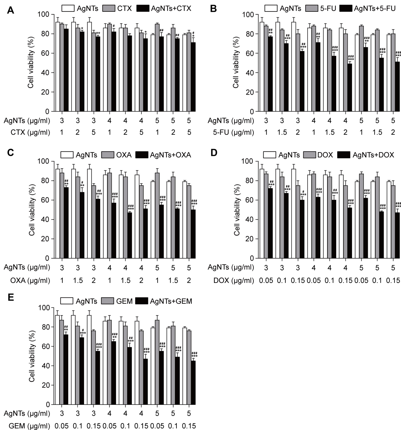
Figure 4 Effect of AgNTs, chemotherapeutics or their combinations on C6 cells viability. Notes: The cell viability of C6 cells treated with various concentrations of AgNTs, CTX, 5-FU, OXA, DOX or GEM, or AgNTs plus one of these drugs in different AgNTs-to-drug concentration ratios for 24 h was determined by the MTT assay. The corresponding cell viability is shown in (A–E). Data are represented as the mean ± SD obtained from three independent experiments. When compared with the corresponding single AgNTs group, * P < 0.05, ** P < 0.01, *** P < 0.001. When compared with the corresponding single drug group, # P < 0.05, ### P < 0.01, #### P < 0.001. Abbreviations: AgNTs, silver nanotriangles; CTX, cyclophosphamide; 5-FU, 5-fluorouracil; OXA, oxaliplatin; DOX, doxorubicin; GEM, gemcitabine; MTT, 3-(4,5-dimethylthiazol-2-yl)-2,5-diphenyltetrazolium bromide; SD, standard deviation.
