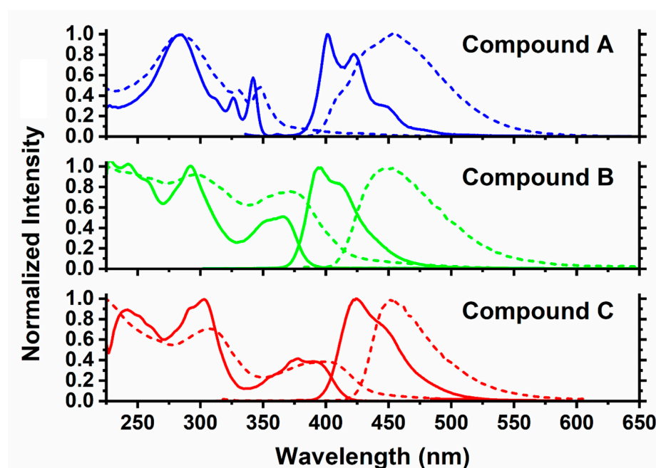
Figure 5. Normalized UV-vis absorption and fluorescence spectra of compound A, B, and C in DCM solutions (1 \mu\text{M} , solid lines) and neat films (dashed lines).
