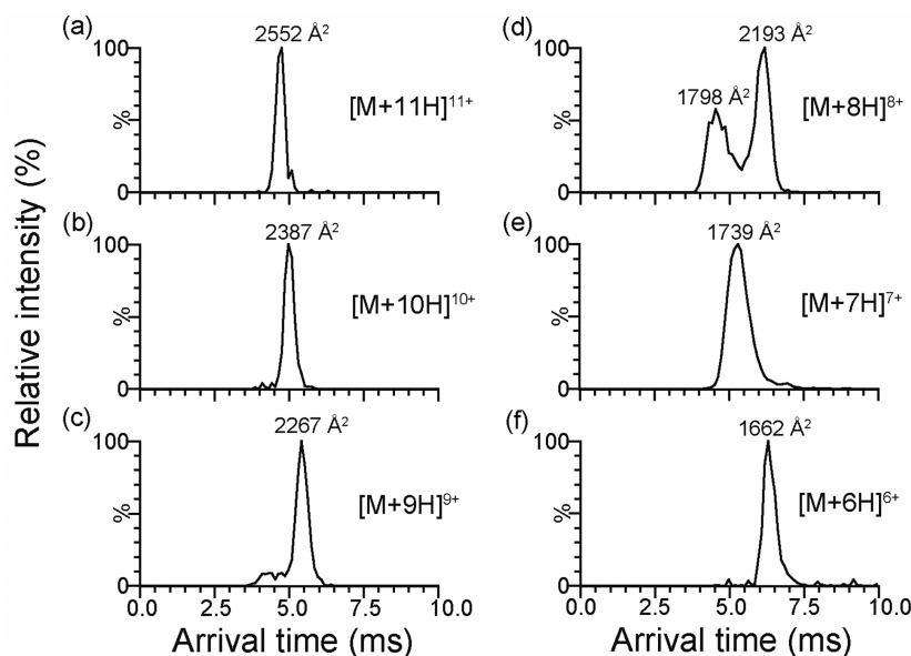
Figure 2. Ion arrival time distribution (ATD) plots obtained from the “native-like” HEWL sample for charge states 11 + to 6 + (a–f), with TW CCS N 2 noted for each peak maximum. Each plot was generated from an approximately ±1.5 Da window around the [M + nH] n+ peak. The charge states 11 + to 9 + (a–c) indicate unfolded structures, whereas 7 + and 6 + (e, f) are indicative of folded structures, evidenced by substantially smaller TW CCS N 2 . The ATD plot of the 8 + charge state (d) displays ion populations of both conformations.
