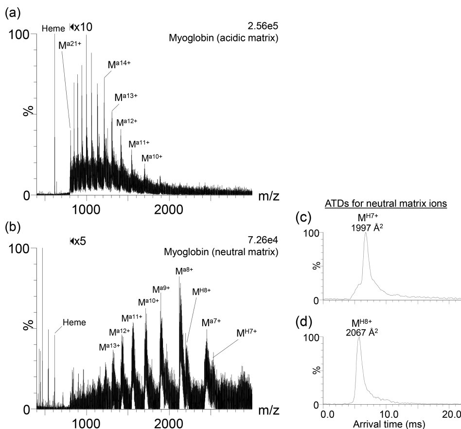
Figure 3. AP-(MA)LDI mass spectra for myoglobin obtained from liquid samples using the acidic matrix (a) and neutral matrix (b). Substantially different CSDs were observed. The apo-form of myoglobin (M a ) was readily detected for both matrices, whereas the heme-binding holo-form (M H ) was only detected with the neutral matrix at lower charge states. The relative abundance of heme is also lower for the analysis under “native-like” conditions. The TW CCS N 2 for the 7 + (c) and 8 + (d) holo-form ions correspond closely to previously reported values. 21
