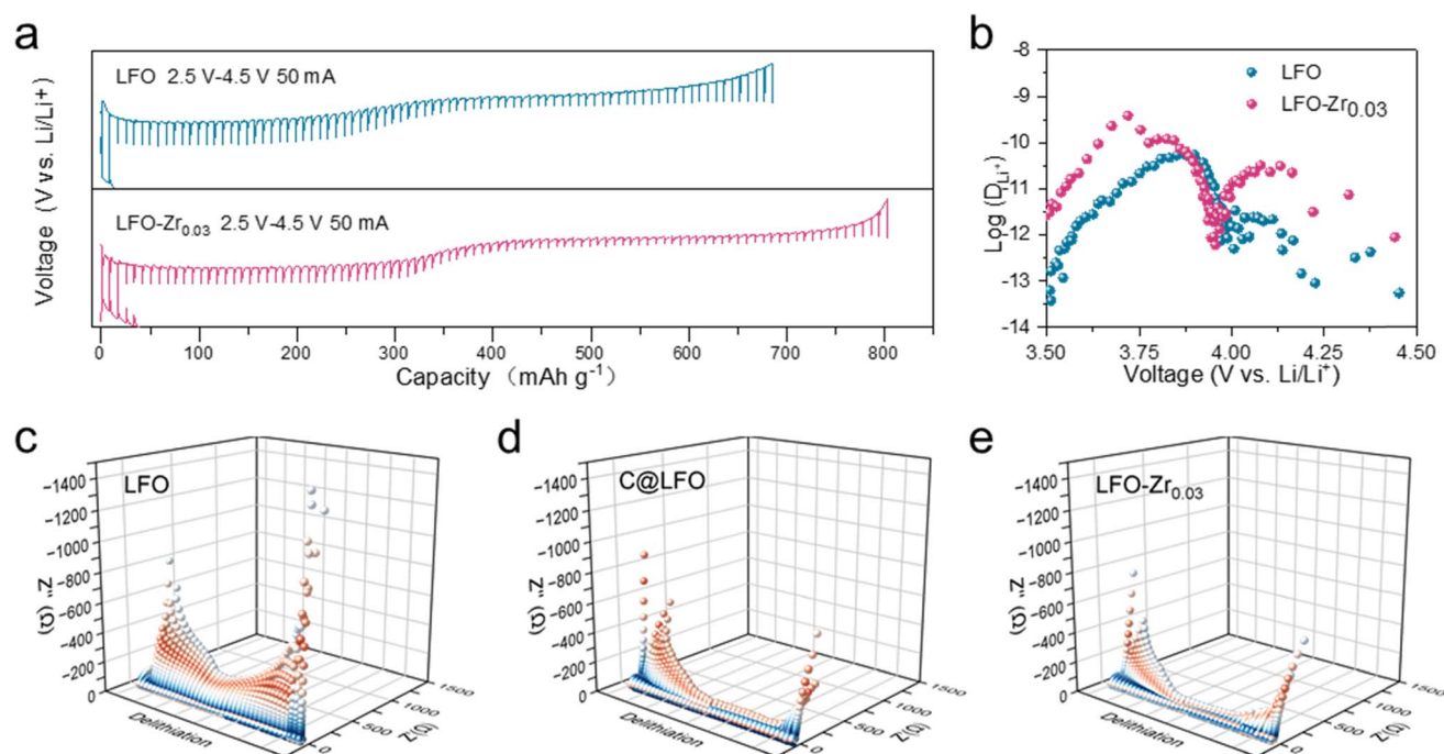
Fig. 4 Kinetic properties of LFO and LFO-Zr 0.03 electrodes. (a) Galvanostatic intermittent titration technique (GITT) profiles and (b) the \log(D_{\text{Li}^+}) -potential plots during charge processes. The in situ EIS of LFO (c), C@LFO (d) and LFO-Zr 0.03 (e) during the initial de-lithiation process.
