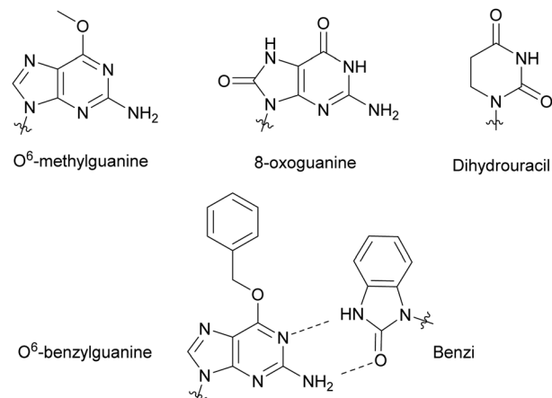
Fig. 4 Nucleobase modifications relevant to DNA damage present in NTPs, utilized to study DNA and RNA repair mechanisms and DNA adduct detection.
