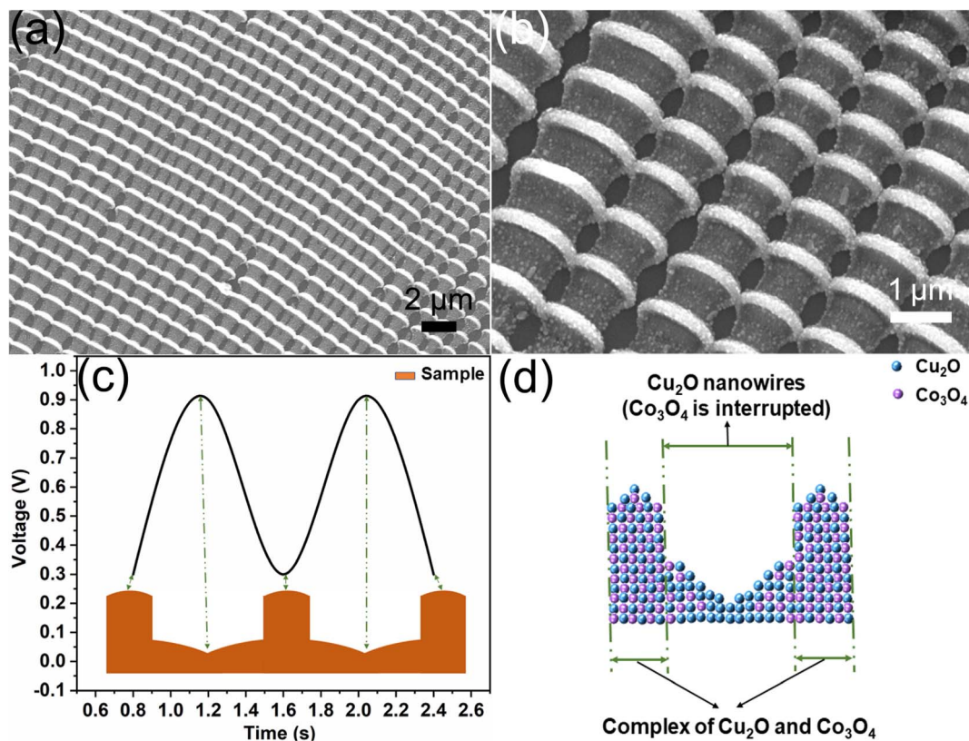
Fig. 2 (a and b) SEM images of Cu 2 O/Co 3 O 4 nanoarrays. (c) Relationship between the sample growth and semi-sine deposition voltage. (d) The distribution of Cu 2 O and Co 3 O 4 in one cycle on the longitudinal section.
