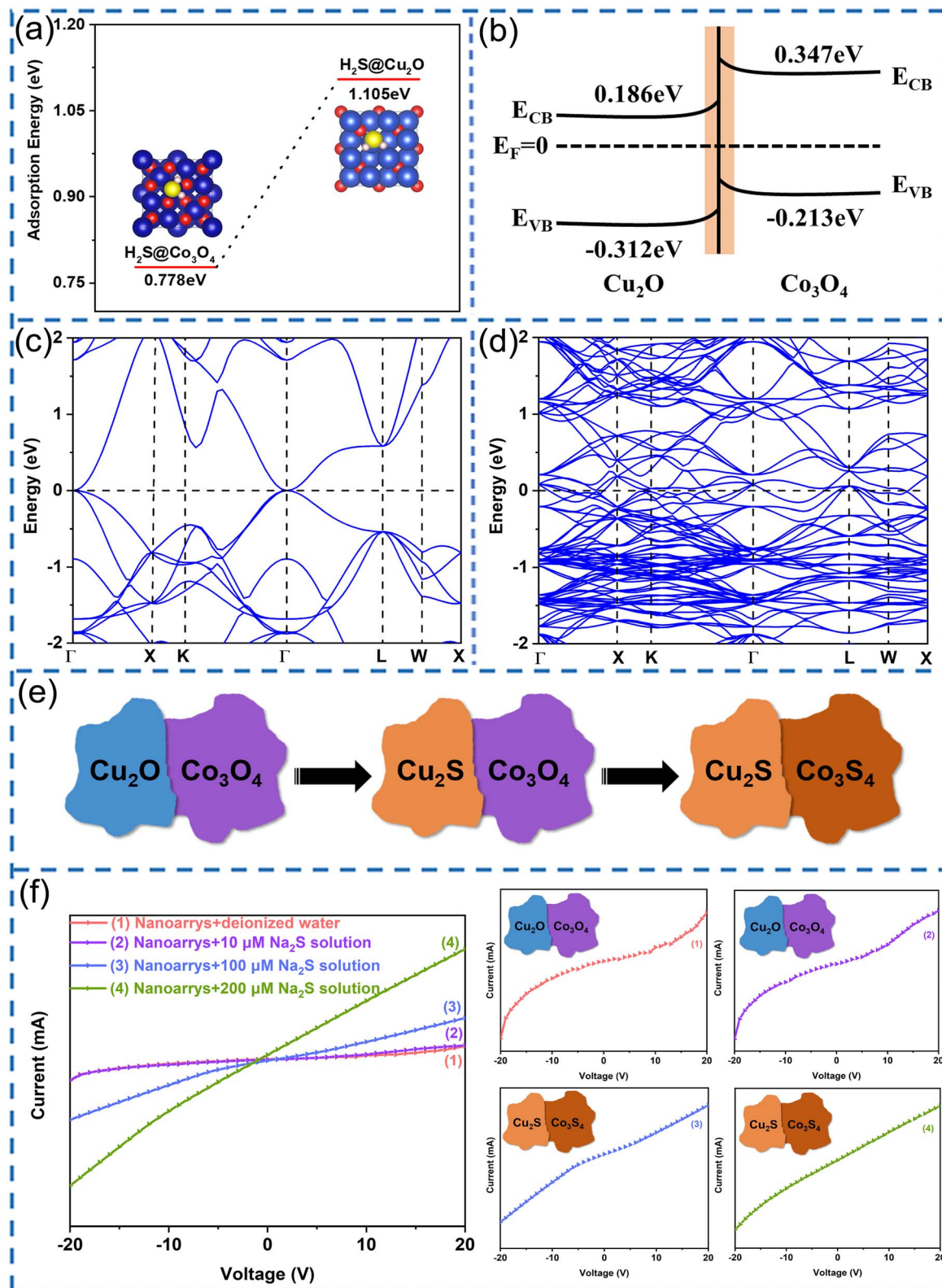
Fig. 8 (a) The adsorption energy of \text{H}_2\text{S}@\text{Cu}_2\text{O} and \text{H}_2\text{S}@\text{Co}_3\text{O}_4 . (b) Energy level diagram of \text{Cu}_2\text{O} and \text{Co}_3\text{O}_4 . The band structure of (c) \text{Cu}_2\text{S} and (d) \text{Co}_3\text{S}_4 . (e) Schematic of the evolution of \text{Cu}_2\text{O}/\text{Co}_3\text{O}_4 nanoarrays after reaction with \text{H}_2\text{S} . (f) I - V curves of the sensors for different concentrations of \text{Na}_2\text{S} solution.
