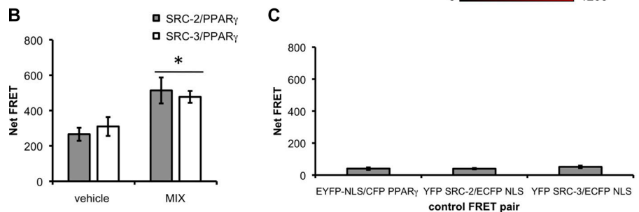
Figure 5. SRC-2 and SRC-3 interact with PPAR \gamma in a differentiation-independent manner. (A) seFRET was used to evaluate the interactions between CFP-PPAR \gamma 2/YFP SRC-2 or CFP-PPAR \gamma 2/YFP SRC-3 after exposure to either vehicle (DMSO) or MIX for 2 h in wild-type HeLa cells. Representative images are shown from one experiment for a single channel (CFP or YFP) with the calculated FRET image. Bars, 10 \mu m. (B) For each cell, the net FRET between CFP-PPAR \gamma 2 and YFP-SRC was determined using the softWoRx user interface. FRET was measured within nucleoplasmic regions of interest only. (C) Control plasmids, ECFP or EYFP fused to a NLS sequence, were coexpressed, and FRET was determined. On average, CFP-PPAR \gamma 2/YFP-SRC FRET signals were 8–20 \times greater than those measured in vector control experiments ( n \geq 22 cells measured over three independent experiments; *, P < 0.05 compared with vehicle treatment). FRET signals were scaled between minimum and maximum signals (0–1,200 pixels), and intensity was colored as shown. Error bars indicate SEM.
