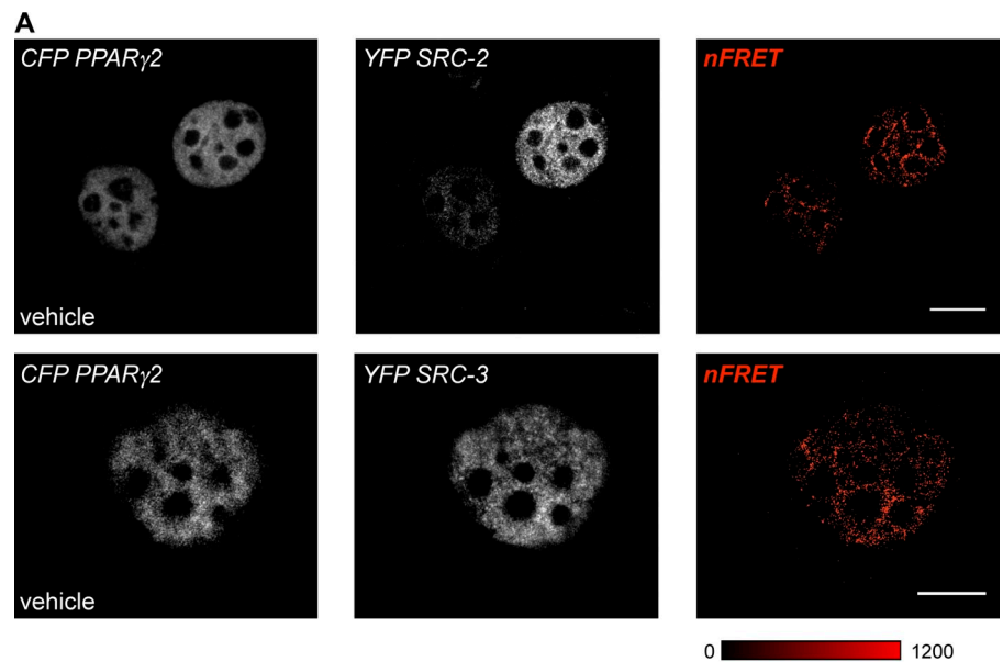
Figure 5. SRC-2 and SRC-3 interact with PPAR \gamma in a differentiation-independent manner. (A) seFRET was used to evaluate the interactions between CFP-PPAR \gamma 2/YFP SRC-2 or CFP-PPAR \gamma 2/YFP SRC-3 after exposure to either vehicle (DMSO) or MIX for 2 h in wild-type HeLa cells. Representative images are shown from one experiment for a single channel (CFP or YFP) with the calculated FRET image. Bars, 10 \mu m. (B) For each cell, the net FRET between CFP-PPAR \gamma 2 and YFP-SRC was determined using the softWoRx user interface. FRET was measured within nucleoplasmic regions of interest only. (C) Control plasmids, ECFP or EYFP fused to a NLS sequence, were coexpressed, and FRET was determined. On average, CFP-PPAR \gamma 2/YFP-SRC FRET signals were 8–20 \times greater than those measured in vector control experiments ( n \geq 22 cells measured over three independent experiments; *, P < 0.05 compared with vehicle treatment). FRET signals were scaled between minimum and maximum signals (0–1,200 pixels), and intensity was colored as shown. Error bars indicate SEM.
