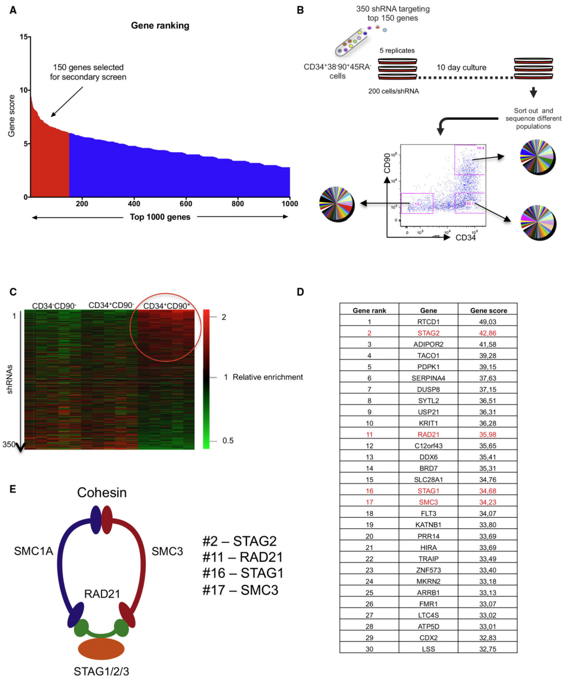
Figure 2. A Targeted Screen in Highly Enriched HSC Populations Identifies Cohesin Genes as Candidate Regulators of Renewal and Differentiation
