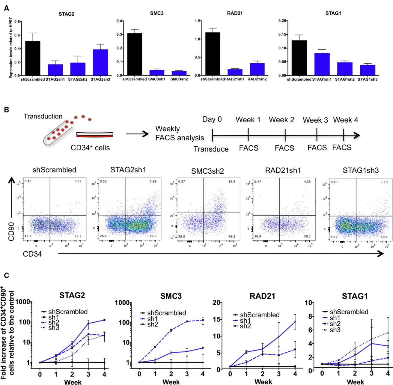
Figure 3. Knockdown of Cohesin Genes Impairs Differentiation and Expands Primitive Cells Ex Vivo
