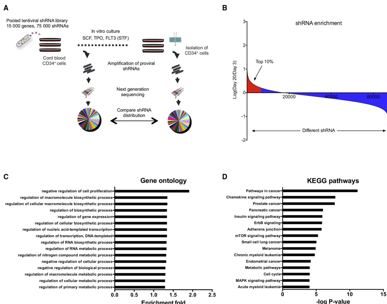
Figure 1. Genome-wide RNAi Screen in Primitive Human Hematopoietic Cells Defines Genes and Pathways Associated with Cancer Progression and Cell Proliferation
