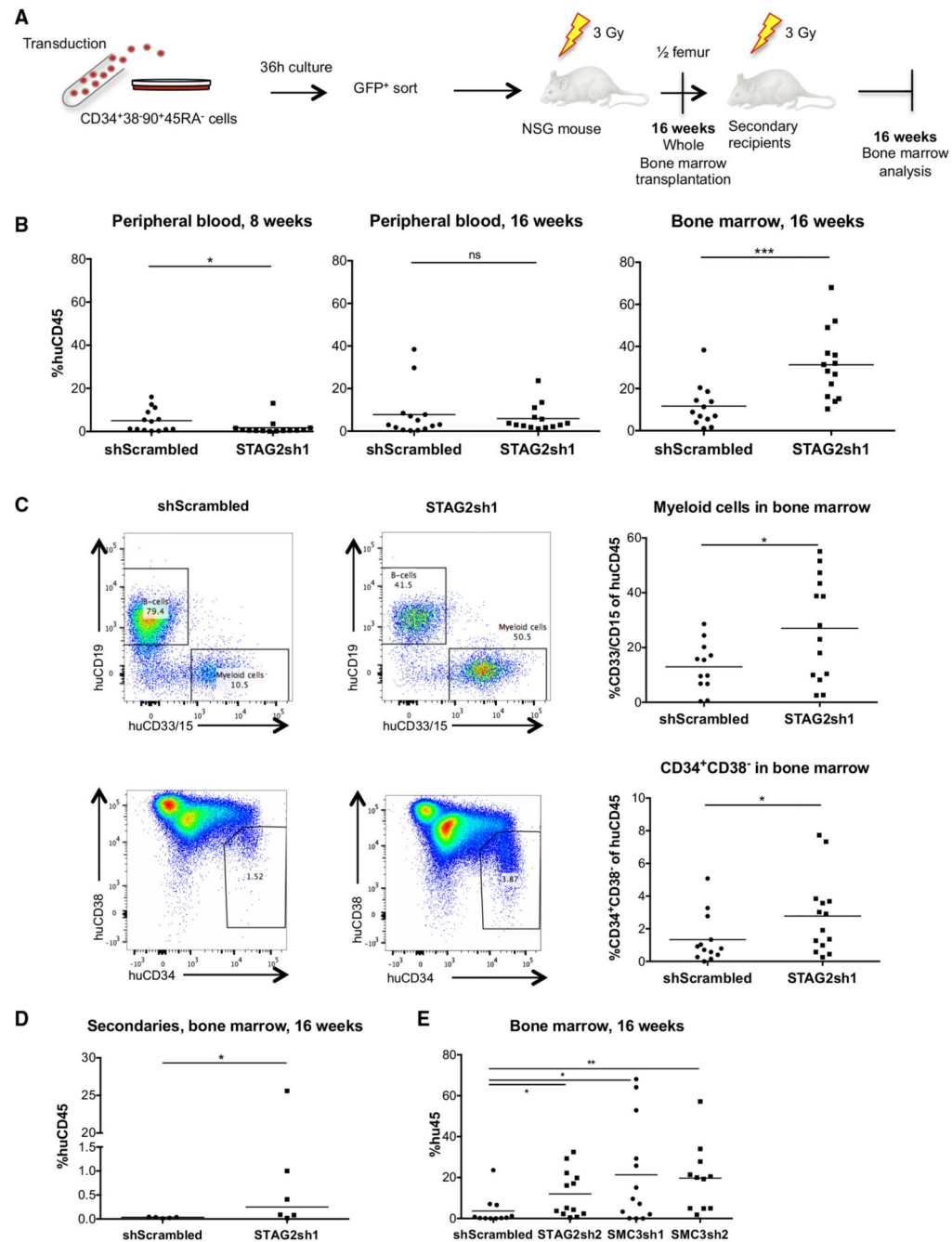
Figure 4. Cohesin-Deficient HSCs Show Increased Reconstitution Potential following Transplantation to Primary and Secondary Immunodeficient Mice
