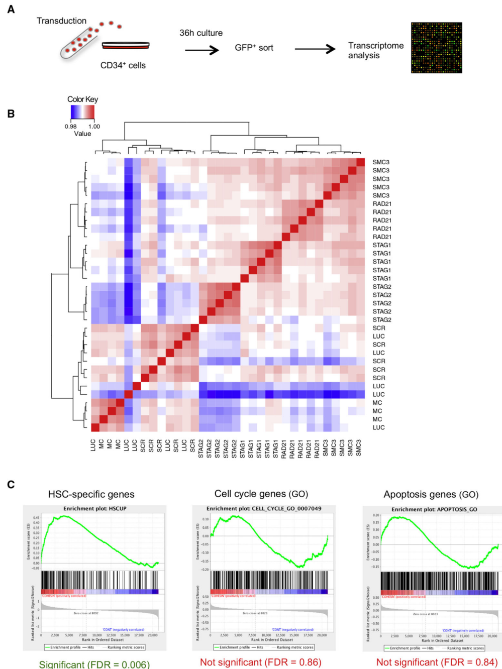
Figure 5. Silencing of Cohesin Genes Results in Immediate Transcriptional Changes with a Shift toward a More HSC-like Gene Expression Signature
