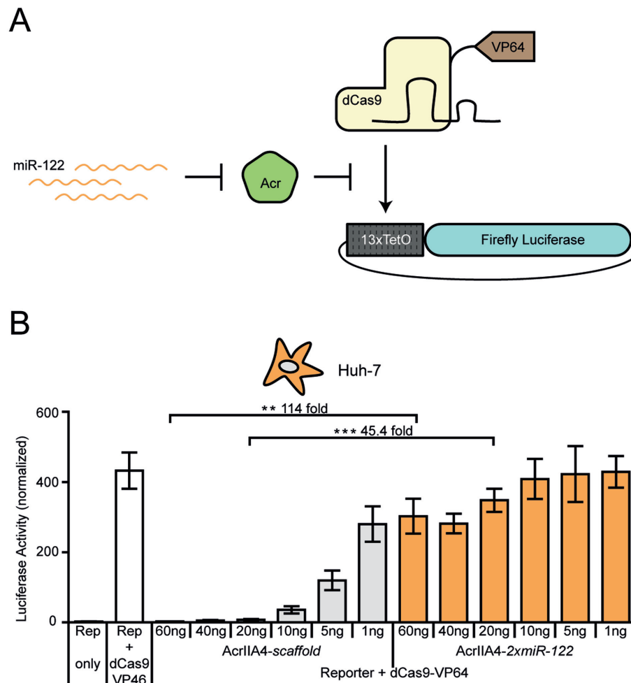
Figure 3. MiR-122-dependent gene activation via SpyCas9 -VP64. (A) Schematic of miR-122-dependent activation of luciferase reporter expression. MiR-122-dependent knockdown of AcrIIA4 results in SpyCas9 -VP64 activity and thus luciferase expression. (B) Huh-7 cells were co-transfected with vectors encoding SpyCas9 -VP64, a luciferase reporter driven by a minimal promoter preceded by tet operator (TetO) sites, a TetO-targeting sgRNA and AcrIIA4- miR-122 or AcrIIA4- scaffold construct (as control), followed by a luciferase assay. During transduction, the Acr vector dose was varied as indicated. Data are means \pm s.e.m. ( n = 4 independent experiments). ** P < 0.01 , *** P < 0.001 , by two-sided Student's t -test with Bonferroni correction. For all doses, precise P -values are shown in Table 1 (Material and Methods).
