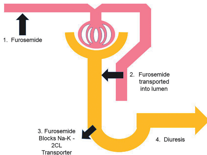
Figure 2. Testing of renal tubular integrity with the furosemide stress test in early AKI. In order for a brisk urinary response to furosemide there are four components that must be achieved. 1. Furosemide enters the blood stream and then must bind to albumin. 2. Active secretion by proximal tubule from the basolateral membrane to the lumen by the hOAT system. 3. Transport of the furosemide in the lumen dissolved in the glomerular filtrate transported to the TAL and binding to the Na- K-2Cl apical transporter. 4. Resultant diuresis.
