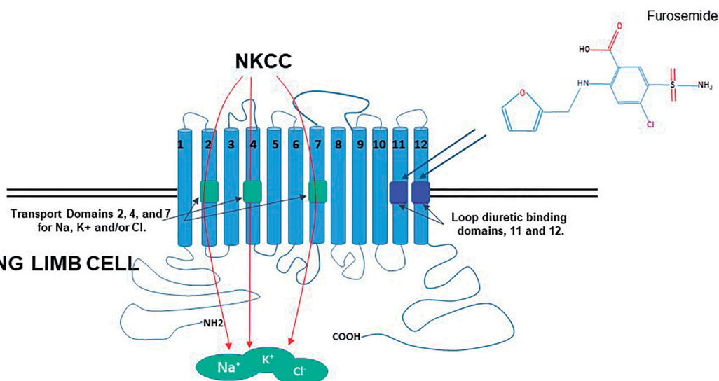
Figure 1. Schematic diagram showing the 12 transmembrane domain Na-K-2Cl (NKCC) transporter in the thick ascending limb of the loop of Henle. Loop diuretics bind to the chloride-binding site (portions of the transmembrane domains 11 and 12) resulting in obstruction and subsequent inhibition of the NKCC-2 transporter domains 2, 4, and 7 transport Na, K, and/or Cl.
