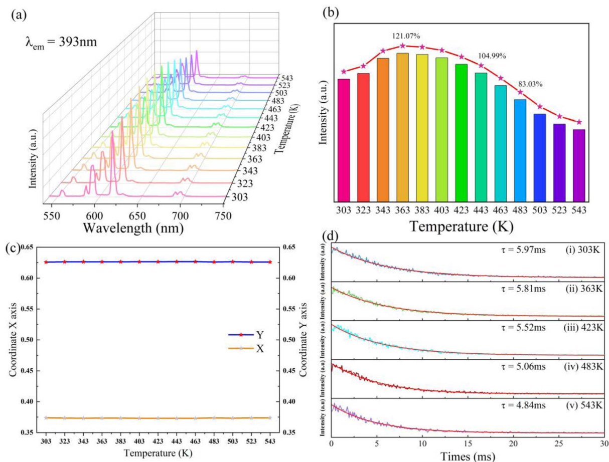
Fig. 10 (a) Emission spectrum of \text{NaYF}_4:0.065\text{Eu}^{3+},0.003\text{Dy}^{3+} at a distinct temperature. (b) Luminous intensity of the primary emission peak at temperatures 303 K to 543 K. (c) Change of CIE color coordinates from 303 K to 543 K. (d) Decay measured at 303 K, 363 K, 423 K, 483 K, and 543 K.
