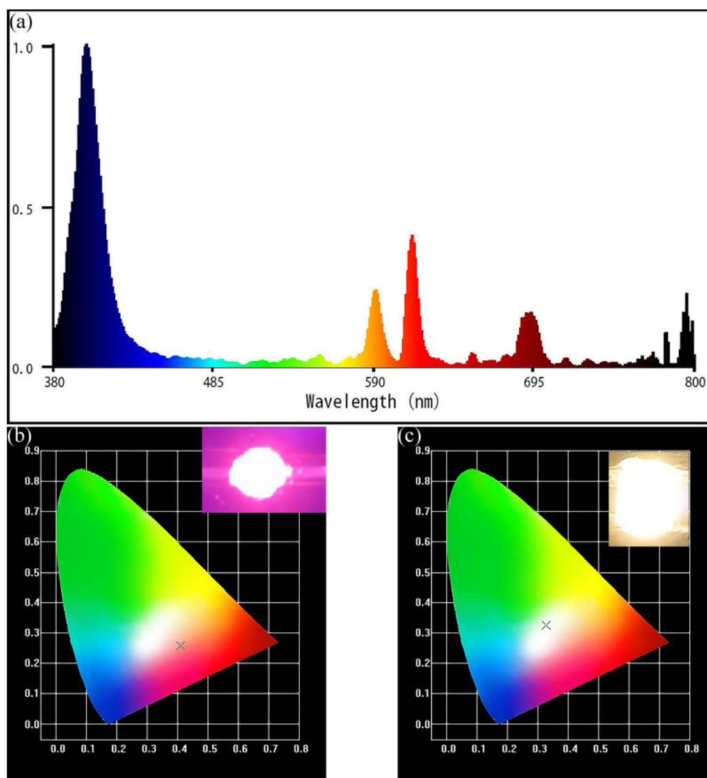
Fig. 12 (a) Luminescent performance of prototype LEDs ( \text{NaYF}_4:0.065\text{Eu}^{3+},0.003\text{Dy}^{3+} + 395 nm UV chip) and luminescent graph. (b) The CIE chromaticity diagram of fabricated LEDs. (c) The CIE coordinate and fabricated WLEDs combining the \text{YAG}:\text{Ce}^{3+} yellow phosphor with \text{NaYF}_4:0.065\text{Eu}^{3+},0.003\text{Dy}^{3+} phosphor and 395 nm UV chip.
