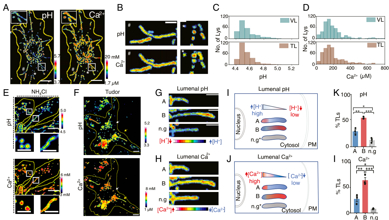
Fig. 4. Heterogeneity of ionic gradient within TLs. (A) pH and \text{Ca}^{2+} images of CalipHluor2.0 -labeled RAW 264.7 cells treated with Tudor . (B) pH and \text{Ca}^{2+} maps of TLs and VLs. (C and D) Lysosomal (C) pH and (D) \text{Ca}^{2+} distributions in VLs of dsDNA-treated RAW 264.7 and TLs of Tudor -treated cells (~20 cells, ~300 VLs, ~100 TLs). (E) pH and \text{Ca}^{2+} images of Tudor -treated RAW 264.7 cells in the presence of 10 mM \text{NH}_4\text{Cl} . (F) pH and \text{Ca}^{2+} images of Tudor -treated RAW 264.7 cells showing both VLs and TLs. (G and H) pH and \text{Ca}^{2+} maps of TLs. (I and J) Schematic of the different TL populations according to their luminal gradients and orientation in the cell. n.g.: no gradient. (K and L) Percentage of TL populations ( N = 20 cells, n = 100 TLs). *** P < 0.0005 ; ** P < 0.005 ; * P < 0.05 . (Scale bars, 10 \mu\text{m} ; zoomed scale bars, 2 \mu\text{m} .)
