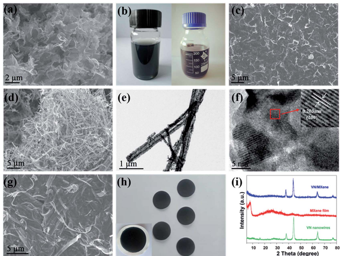
Fig. 1 (a) SEM images of the prepared Ti_3C_2T_x nanosheets. (b) Photographs of Ti_3C_2T_x -water dispersion and VN- Ti_3C_2T_x -water dispersion. (c) SEM images of the prepared Ti_3C_2T_x film. (d) SEM image of the prepared VN nanowires. (e) TEM and (f) HRTEM images of VN nanowires. (g) SEM images of VN/MXene composite film. (h) Photographs of free-standing VN/MXene composite film electrode. (i) XRD patterns of the Ti_3C_2T_x film, VN nanowires and VN/MXene composite, respectively.
