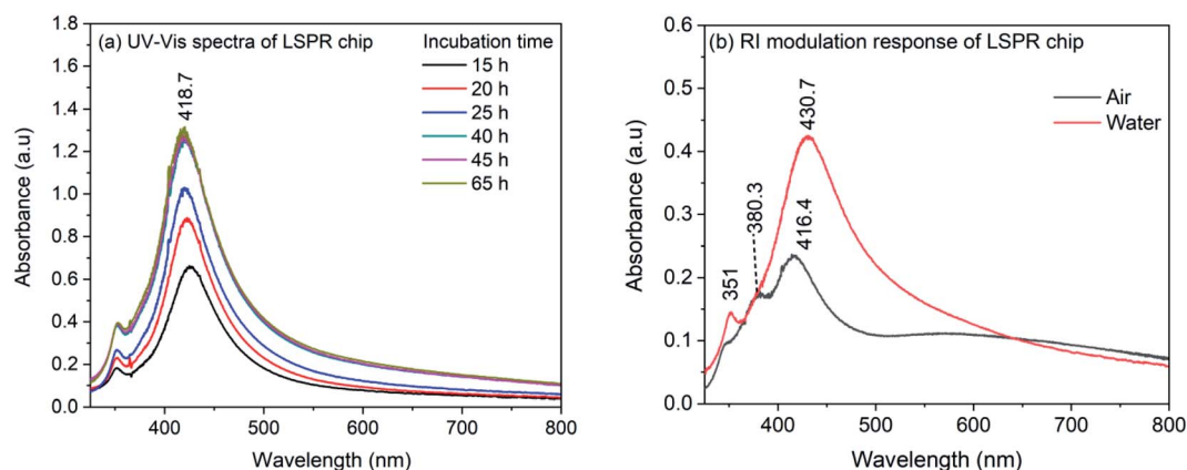
Fig. 2 (a) UV-Vis spectra of AgNCs LSPR chip recorded for different incubation time (b) UV-Vis spectra of LSPR chip in air and in water.
