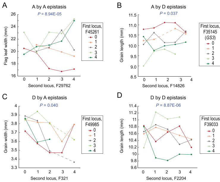
Figure 5. Patterns of interactions of the four epistasis types displayed by various two-locus combinations. P value in each panel represents the statistical probability for relative epistasis. The vertical axis represents phenotypic value, and genomic types of 0–4 represent N : 9 homoeolog ratios of 0 : 4, 1 : 3, 2 : 2, 3 : 1 and 4 : 0, respectively.
