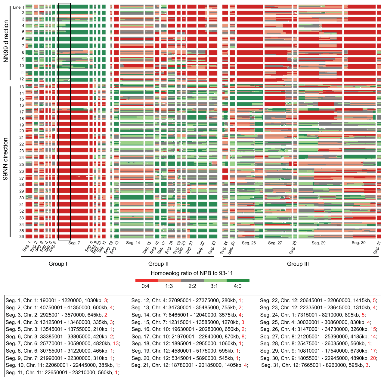
Figure 3. Heatmaps showing the genomic compositions of 31 cytonuclear compatibility-related chromosomal segments being strongly selected for from all of the 202 genome-re-sequenced S_4 tetraploid individuals. The different colors show the different genomic types, e.g. the orange color represents that the homoeologous ratio between NPB and 93-11 in this given locus is 1 : 3. Each row represents one tetraploid individual, the 31 columns indicate 31 chromosomal segments. Cross direction and line names are labeled on the left of the rows. Information of segment ID, chromosome, genomic location, segment size and the number of cytonuclear molecular interaction genes is given in the lower panel. The framed box in Seg. 7 denotes a 1787 kb genomic region retaining at least one maternal copy in all (100%) individuals.
