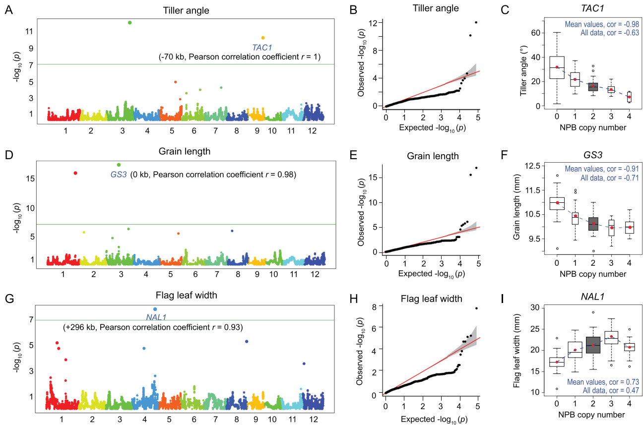
Figure 4. GWAS of tiller angle, grain length and flag-leaf width with the additive model by FarmCPU R scripts. (A), (D) and (G) are Manhattan plots, wherein the green lines represent thresholds based on Bonferroni tests, with genes controlling the given trait labeled in blue below the corresponding locus. (B), (E) and (H) are Quantile-Quantile plots of p-values. (C), (F) and (I) are boxplots showing the additive relationship between phenotype and NPB copy number in each of the three genes.
