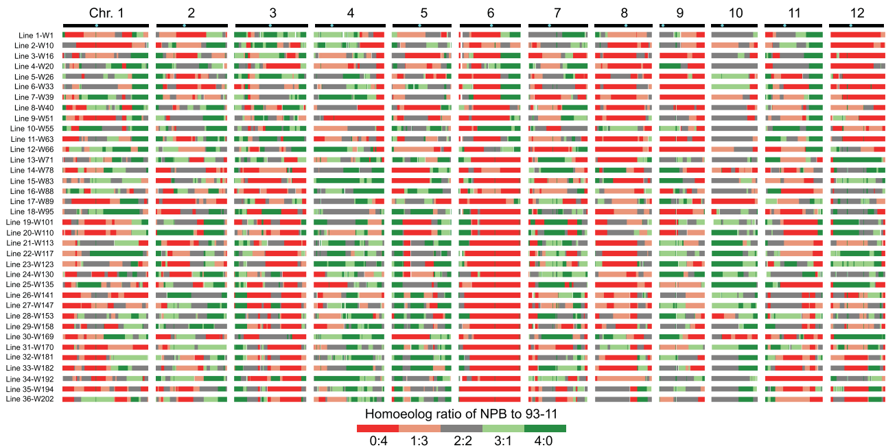
Figure 2. Heatmaps depicting the genomic landscapes of 36 randomly selected S4 euploid tetraploid individuals from 36 selfed lines (Supplementary Fig. S1). Different colors denote different homoeolog compositions, where orange representing NPB homoeolog percentage at a given locus is 25%, i.e. the homoeolog ratio between NPB and 93-11 is 1 : 3. Each row represents one tetraploid individual, the 12 columns represent the 12 chromosomes in the rice genome, and the light blue dots denote centromeres.
