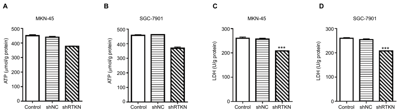
Figure S2 RTKN shRNA decreased ATP content and LDH level in GC cells.
